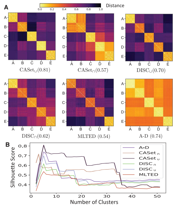
Fig. 4. (A) Inter-dataset distance heatmaps of five tree families in the OncoLib dataset. The color of each cell represents the distance between two trees. Average silhouette scores for five clusters are displayed in parentheses to quantify clustering tightness and separation. We note that we normalized the A–D distance by dividing by the total number of possible ancestral relationships, so that all distances were in the interval [0, 1]. While this results in A–D distances that are all relatively small ( <0.4 ), the families still exhibit clear clustering. (B) Silhouette scores of clustering the 250 trees in the OncoLib dataset with different distance measures
