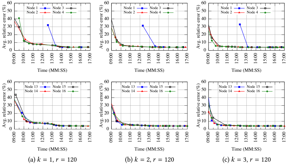
Fig. 21. Dataset S_1 : convergence speed of DiSC on cluster nodes N_1 - N_4 and N_{13} - N_{16} (200M data instances)
