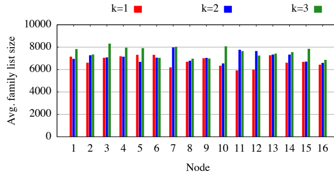
Fig. 14. Dataset S_1 : reduction in the size of the family list at the nodes due to dropping of families in DiSC ( r = 120 )
