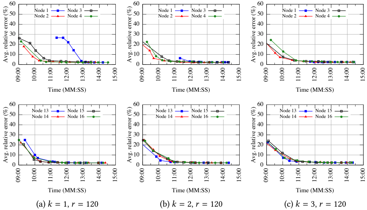
Fig. 24. Dataset HIGGS: convergence speed of DiSC on cluster nodes N_1-N_4 and N_{13}-N_{16} (176M data instances)
