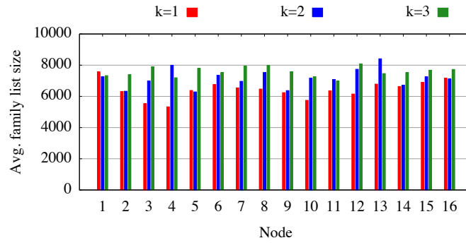
Fig. 16. Dataset S_3 : reduction in the size of the family list at the nodes due to dropping of families in DiSC ( r = 120 )
