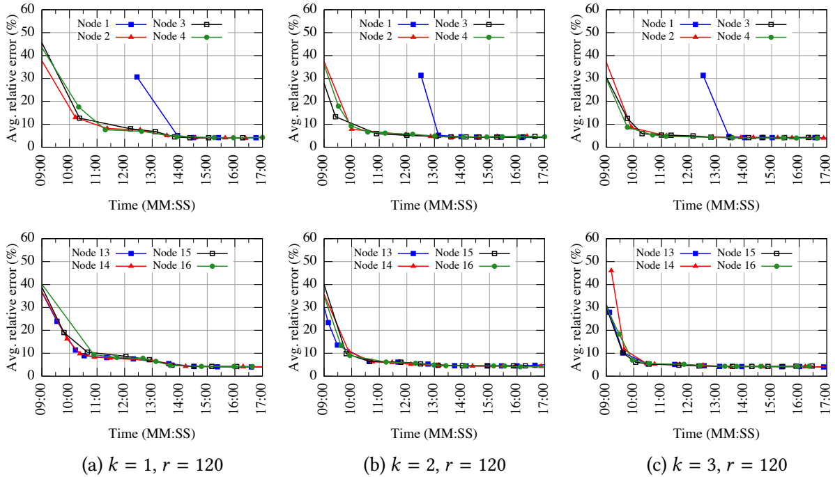
Fig. 23. Dataset S_3 : convergence speed of DiSC on cluster nodes N_1-N_4 and N_{13}-N_{16} (200M data instances)
