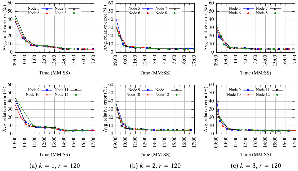
Fig. 11. Dataset S_3 : convergence speed of DiSC on cluster nodes N_5 - N_{12} (200M data instances)
