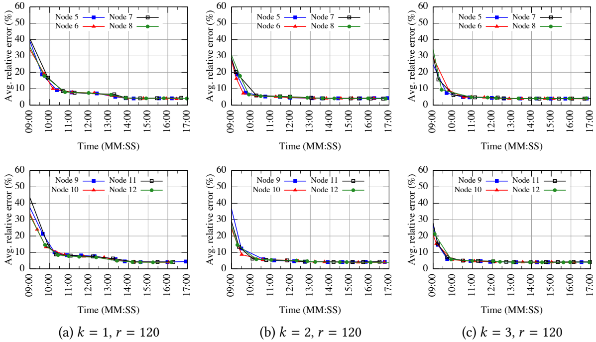
Fig. 9. Dataset S_1 : convergence speed of DiSC on cluster nodes N_5-N_{12} (200M data instances)
