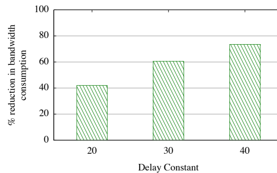
Fig. 19. Reduction in bandwidth due to increase in the delay constant. The results are for the dataset S_2 with r = 120 and k = 2 .
