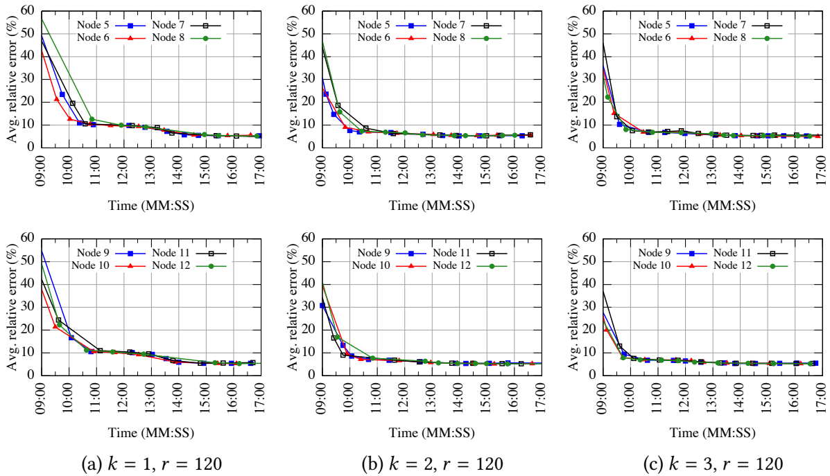
Fig. 10. Dataset S_2 : convergence speed of DiSC on cluster nodes N_5-N_{12} (200M data instances)
