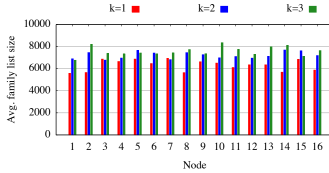
Fig. 15. Dataset S_2 : reduction in the size of the family list at the nodes due to dropping of families in DiSC ( r = 120 )
