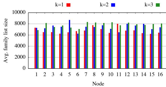
Fig. 17. Dataset HIGGS: reduction in the size of the family list at the nodes due to dropping of families in DiSC ( r = 120 )
