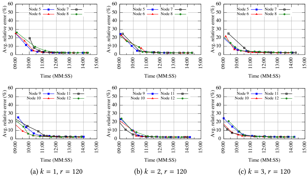
Fig. 12. Dataset HIGGS: convergence speed of DiSC on cluster nodes N_5 - N_{12} (176M data instances)
