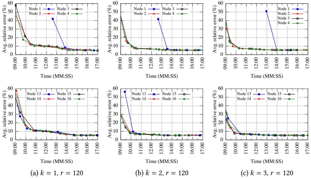
Fig. 22. Dataset S_2 : convergence speed of DiSC on cluster nodes N_1-N_4 and N_{13}-N_{16} (200M data instances)
