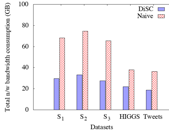
Fig. 20. Comparison of a naive approach and DiSC based on total network bandwidth consumption. We report the results on the five datasets for k = 1 and r = 120 .
