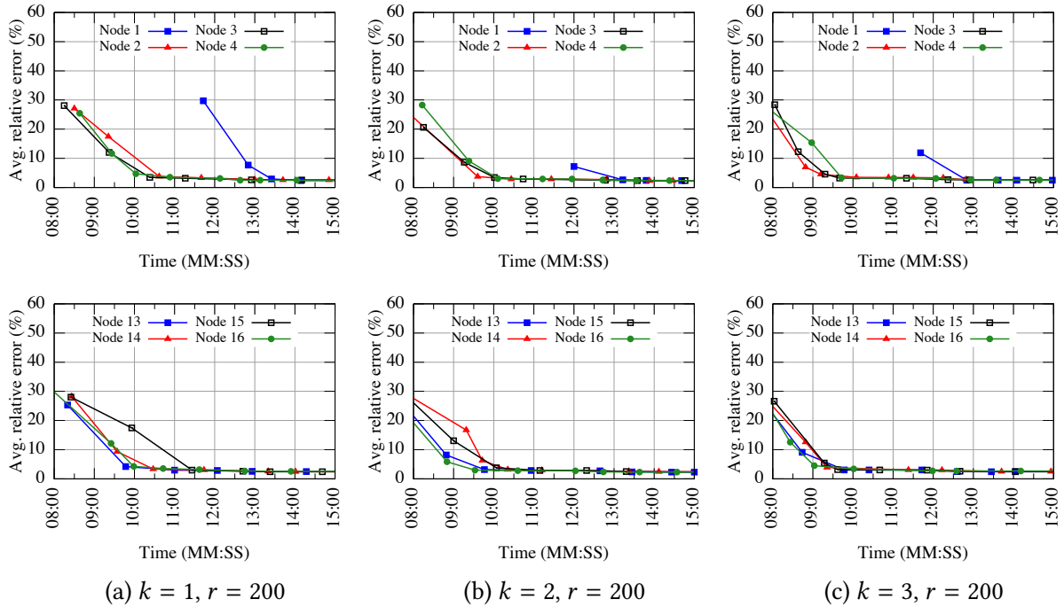
Fig. 25. Dataset Tweets: convergence speed of DiSC on cluster nodes N_1-N_4 and N_{13}-N_{16} (200M data instances)
