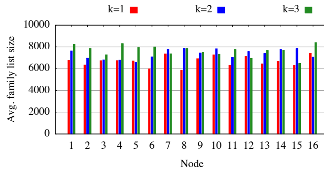
Fig. 18. Dataset Tweets: reduction in the size of the family list at the nodes due to dropping of families in DiSC ( r = 120 ).
