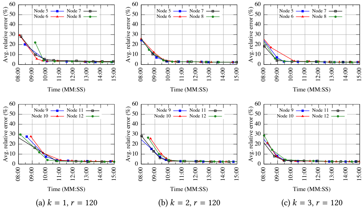
Fig. 13. Dataset Tweets: convergence speed of DiSC on cluster nodes N_5 - N_{12} (200M data instances)
