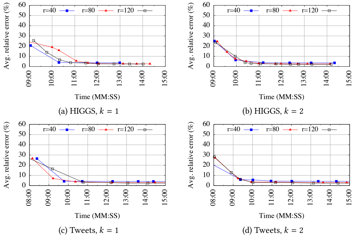
Fig. 8. HIGGS and Tweets: impact of r on the average relative error of the estimates computed by DiSC on a cluster node
