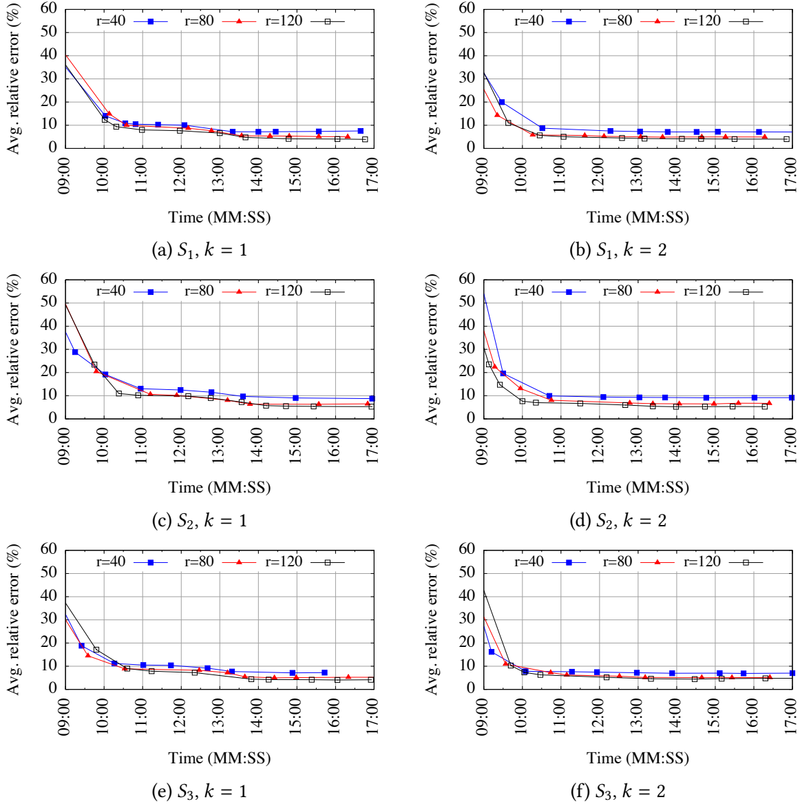
Fig. 7. Synthetic datasets: impact of r on the average relative error of the estimates computed by DiSC on a cluster node
