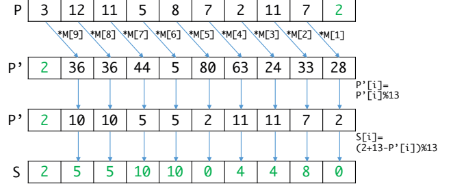
Figure 6. The communication and computing pattern during generation of suffix fingerprints, using the prefix fingerprints of the previous step
