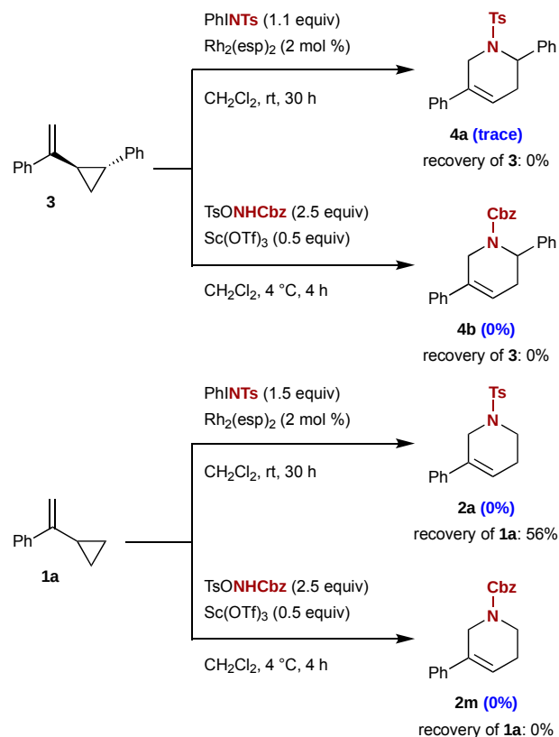
Scheme 2. Control experiments to investigate the complementarity of Sc-promoted and Rh-catalyzed conditions and the role of the nitrene precursor.
