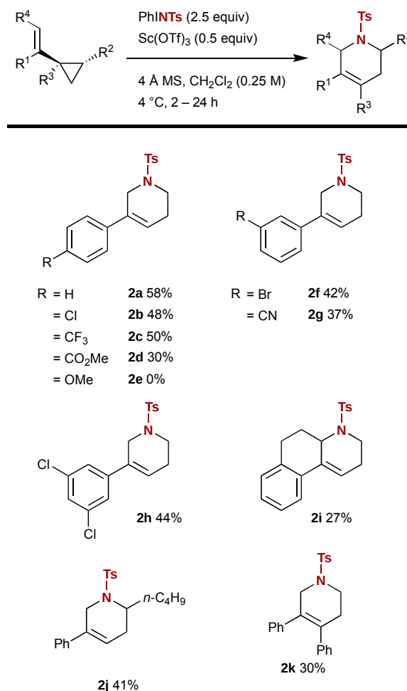
Fig. 1 Scope and limitations of the [5+1] cycloaddition. Yields shown are of isolated products. The substrate was added to a mixture of the other reagents over 1 h. Reactions were monitored by TLC and quenched once full consumption of the substrate was observed.
