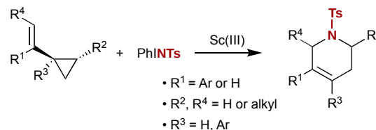
Scheme 1. [5+1] Nitrene-transfer cycloaddition.
