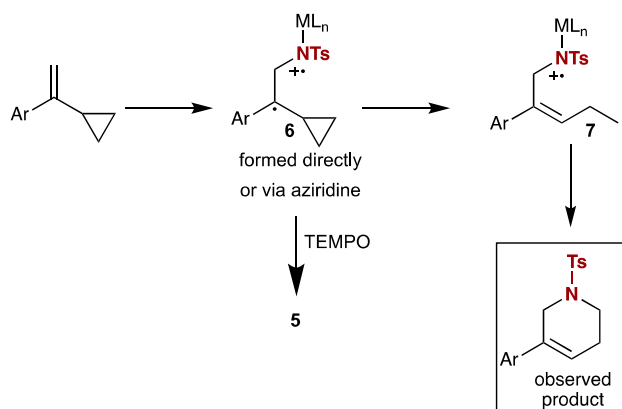
Scheme 3. TEMPO trapping experiment and proposed mechanism for the formation of [5+1] products.
