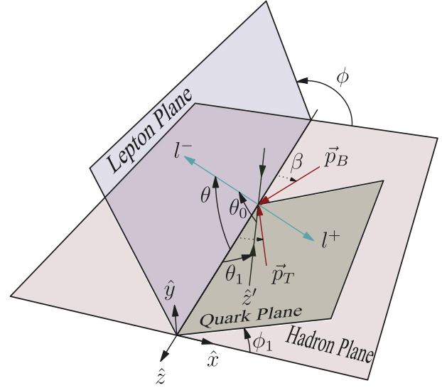
Fig. 1. Definition of the Collins–Soper frame and various angles and planes in the rest frame of \gamma^*/Z or a vector quarkonium. The hadron plane is formed by \vec{p}_B and \vec{p}_T , the momentum vectors of the two interacting hadrons. The \hat{x} and \hat{z} axes of the Collins–Soper frame both lie in the hadron plane with \hat{z} axis bisecting the \vec{p}_B and -\vec{p}_T vectors. The quark ( q ) and antiquark ( \bar{q} ) annihilate collinearly with equal momenta to form \gamma^*/Z or a vector quarkonium, while the quark momentum vector \hat{z}' and the \hat{z} axis form the quark plane. The polar and azimuthal angles of \hat{z}' in the Collins–Soper frame are \theta_1 and \phi_1 . The l^- and l^+ are emitted back-to-back with \theta and \phi as the polar and azimuthal angles for l^- .
