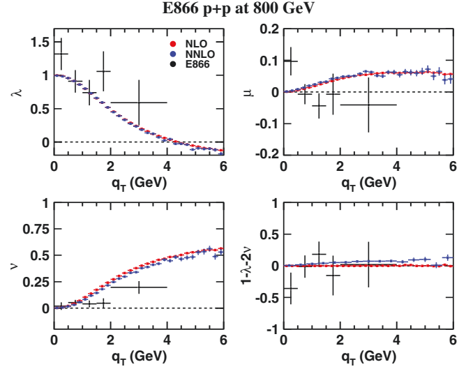
FIG. 5. Comparison of NLO (red points) and NNLO (blue points) fixed-order pQCD calculations with the E866 p + p D-Y data at 800 GeV [15] (black points) for \lambda , \mu , \nu and 1 - \lambda - 2\nu .
