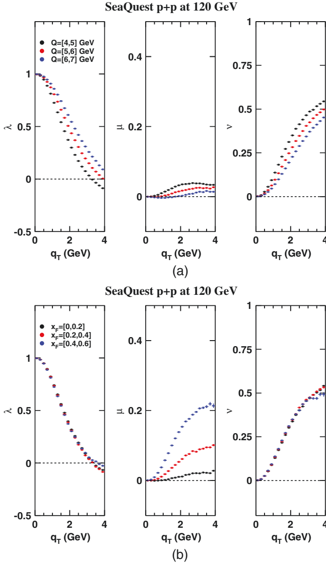
FIG. 8. (a) NLO pQCD results of \lambda , \mu , and \nu as a function of q_T at several Q bins and x_F > 0 for D-Y production off the proton target with 120-GeV proton beam in the SeaQuest experiment. (b) Same as (a) but at several x_F bins and 4 < Q < 9 GeV.
