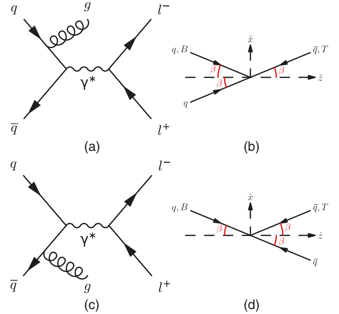
FIG. 13. (a) Feynman diagram for q - \bar{q} annihilation where a gluon is emitted from a quark in the beam hadron. (b) Momentum vectors for q and \bar{q} in the C-S frame before and after gluon emission. The momentum direction of q is now collinear with that of \bar{q} . (c) Feynman diagram for the case where a gluon is emitted from an antiquark in the target hadron. (d) Momenta vectors for q and \bar{q} in the C-S frame before and after gluon emission for diagram (c).
