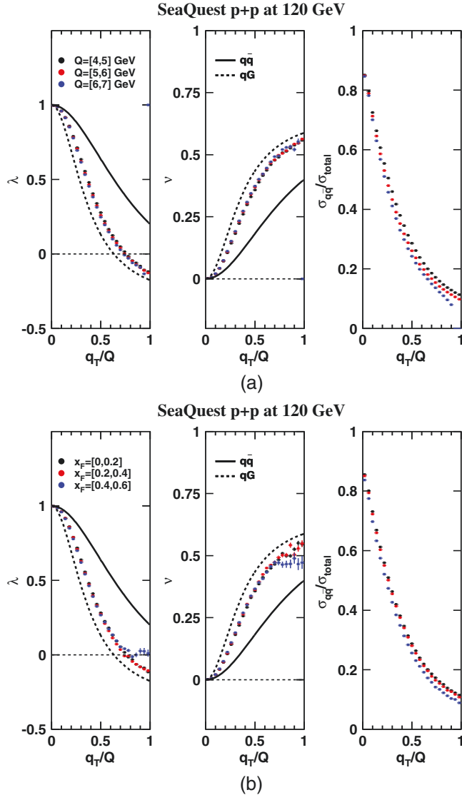
FIG. 10. (a) NLO pQCD results of \lambda , \nu and the fractions of q\bar{q} -process contribution in the total cross sections as a function of scaled transverse momentum q_T/Q for D-Y production off the proton target with 120-GeV proton beam in the SeaQuest experiment. The NLO pQCD expressions of q\bar{q} and qG processes are denoted by the solid and dashed lines respectively. (b) Same as (a) but at several x_F bins and 4 < Q < 9 GeV. It is noted that the rough structure at large q_T/Q region of the results for x_F = 0.4-0.6 (blue points) is likely due to the fluctuation of calculations with Q > 7 GeV near the edge of the phase space. The structure is expected to be removed, if one requires Q < 7 GeV as the top figure.
