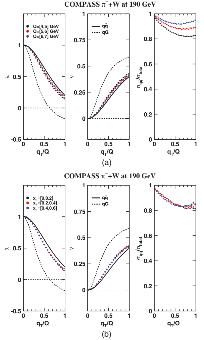
FIG. 9. (a) NLO pQCD results of \lambda , \nu and the fractions of q\bar{q} -process contribution in the total cross sections as a function of scaled transverse momentum q_T/Q for D-Y production off the nuclear tungsten target with 190-GeV \pi^- beam in the COMPASS experiment. The NLO pQCD expressions of q\bar{q} and qG processes are denoted by the solid and dashed lines respectively. (b) Same as (a) but at several x_F bins and 4 < Q < 9 GeV.
