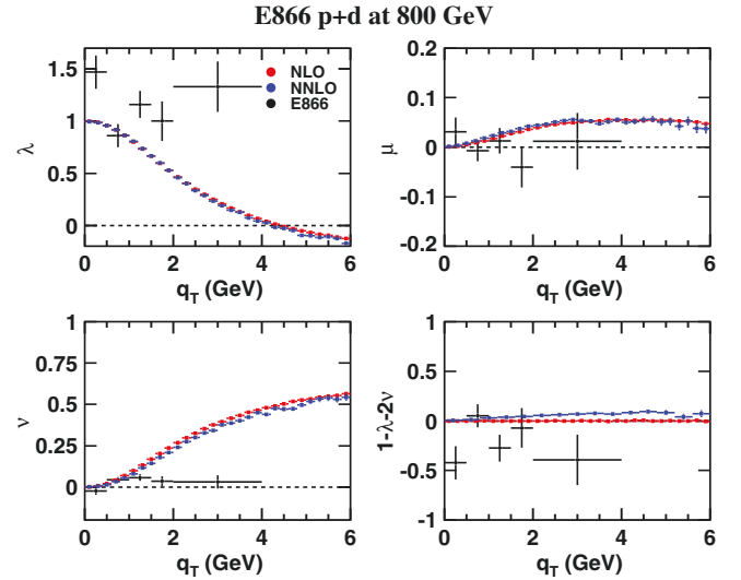
FIG. 6. Same as Fig. 5, but for E866 data [15] with a liquid deuterium target.
