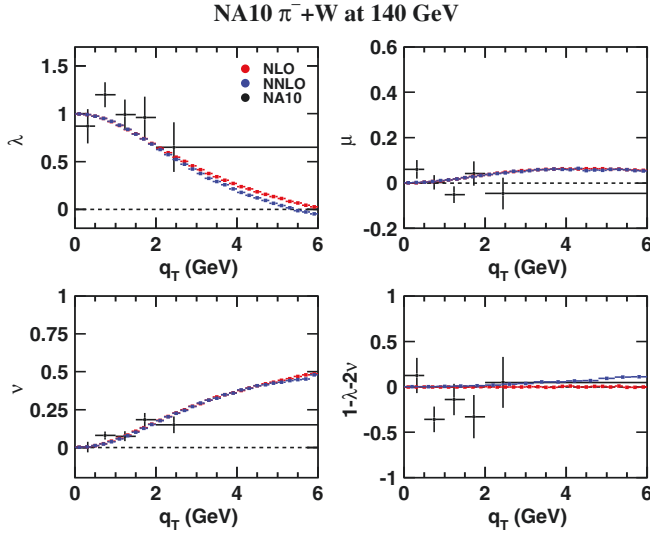
FIG. 1. Comparison of NLO (red points) and NNLO (blue points) fixed-order pQCD calculations with the NA10 \pi^- + W D-Y data at 140 GeV [3] (black points) for \lambda , \mu , \nu and 1 - \lambda - 2\nu .
