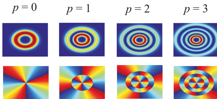
Figure 6. Plots of intensity (top row) and phase (bottom row) in the transverse plane for several l = 3 LG modes with different p values. In addition to the intensity zero on the axis, there are p nodal rings on which the amplitude vanishes (the dark blue rings). The phase is discontinuous in the radial direction at each nodal ring, while increasing linearly in the azimuthal direction in each case.
