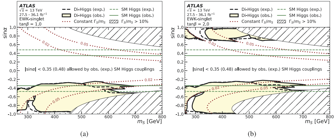
Fig. 6. Excluded regions for the EWK-singlet model for two values of the \tan \beta parameter: (a) \tan \beta = 1 and (b) \tan \beta = 2 . Indirect constraints from SM Higgs coupling measurements [74] are shown with horizontal lines. The dotted lines indicate the separation between regions where the resonance width is larger than 2% and 5% of the resonance mass. The hatch-marked area corresponds to regions that cannot be excluded because the width of the resonance exceeds 10% of the resonance mass, corresponding to the maximum of the experimental mass resolution among all analysed final states.
