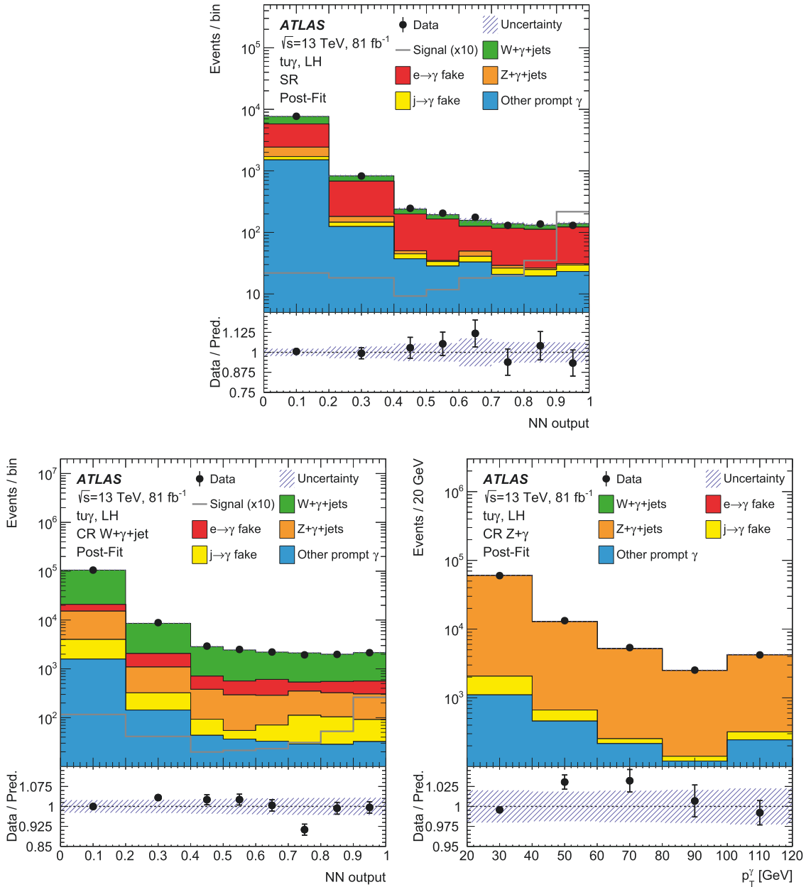
Fig. 2. Post-fit distributions of a background-only fit to the SR and the CRs of the NN output in the SR (top) and the W+γ+jet CR (bottom left) and of the p_T -distribution of the Z+γ CR (bottom right). The last bin of the distribution in the Z+γ CR contains the overflow. In addition, in the SR and in the W+γ+jet CR, the expected signal is overlaid for an effective coupling strength corresponding to the observed limit multiplied by a factor of ten. In the Z+γ CR, the expected signal is not shown, because it is negligible.
