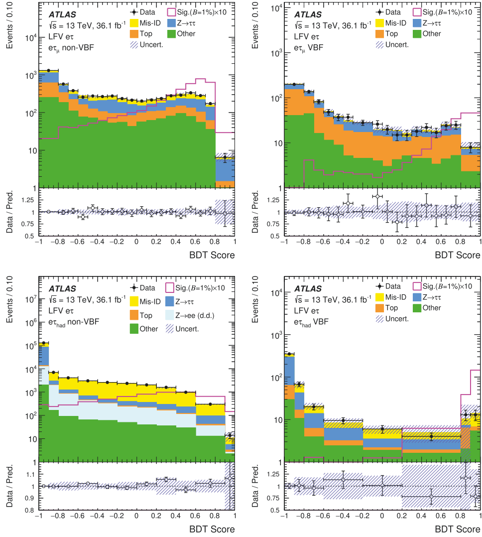
Fig. 2. Distributions of the BDT score after the background+signal fit in each signal region of the e\tau search, with the LFV signal overlaid, normalized with B(H \rightarrow e\tau) = 1\% and enhanced by a factor 10 for visibility. The top and bottom plots display e\tau_\mu and e\tau_{\text{had}} BDT scores respectively, the left (right) column corresponds to the non-VBF (VBF) category. The size of the combined statistical, experimental and theoretical uncertainties of the background is indicated by the hatched bands. The binning is shown as in the statistical analysis.
