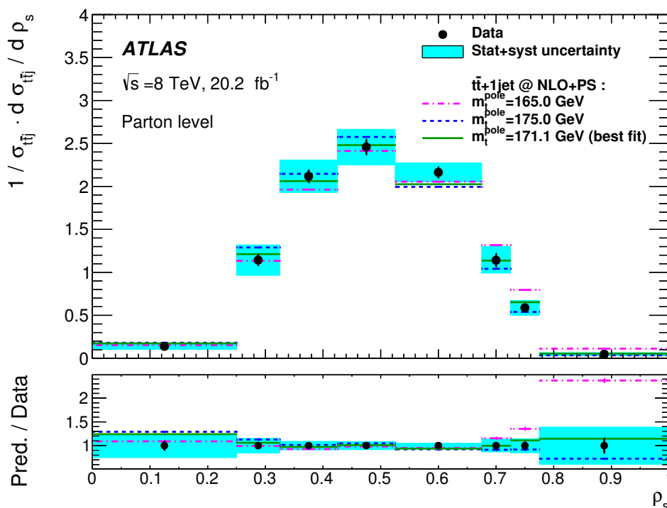
Figure 3. The normalised differential cross section for pp \rightarrow t\bar{t} + 1\text{-jet} production in pp collisions at \sqrt{s} = 8 TeV, as a function of \rho_s . The data are unfolded to the parton level as described in the text. The predictions of the NLO+PS calculation of refs. [25, 83] are shown for a top-quark pole mass of 165 GeV, 175 GeV and 171.1 GeV. Statistical errors are represented by error bars, while the shaded area represents the bin-by-bin sum in quadrature of the statistical and systematics uncertainties, as described in section 8. Bin-by-bin correlations are not shown in the plot.
