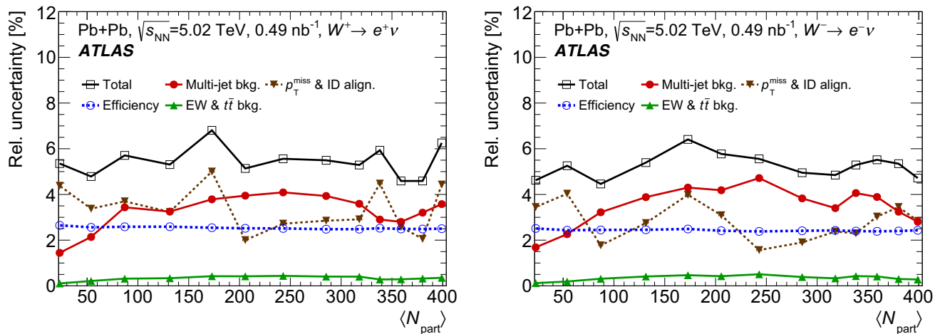
Fig. 5 Relative systematic uncertainties of W^+ (left) and W^- (right) boson production yields measured in the electron decay channel evaluated as a function of \langle N_{\text{part}} \rangle . The total systematic uncertainty is represented by open squares, while other markers represent contributions from individual sources of uncertainty. The uncertainties related
