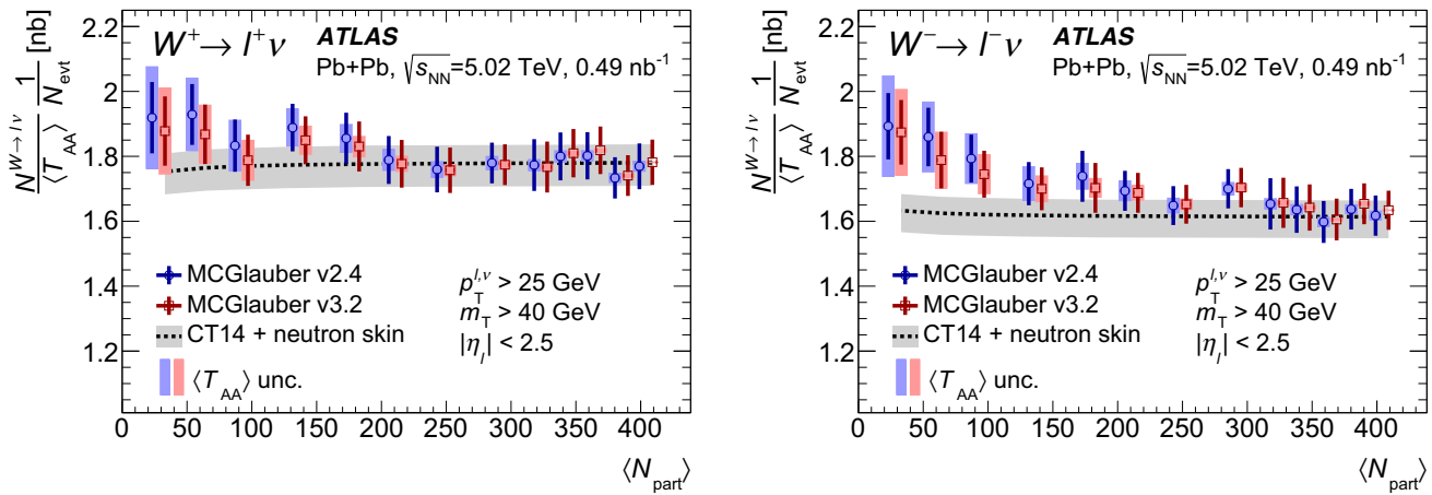
Fig. 13 Comparison of normalised production yields for W^+ (left) and W^- (right) bosons as a function of \langle N_{\text{part}} \rangle for geometric parameters obtained with the MCGlauber code v2.4 and v3.2. The dashed lines show predictions calculated using the CT14 NLO PDF set which incorporate the neutron-skin effect evaluated using the separate radial distributions for protons and neutrons provided by the MCGlauber code
