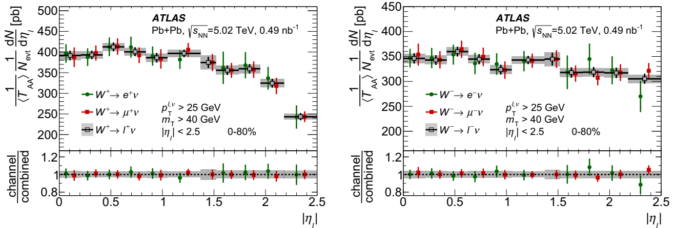
Fig. 7 Differential normalised production yields for W^+ (left) and W^- (right) bosons as a function of absolute pseudorapidity of the charged lepton shown separately for electron and muon decay channels as well as for their combination. Statistical and systematic uncertainties of the combined yields are shown as bars and shaded boxes, respectively. For the individual channels, only the total uncertainties are shown as
