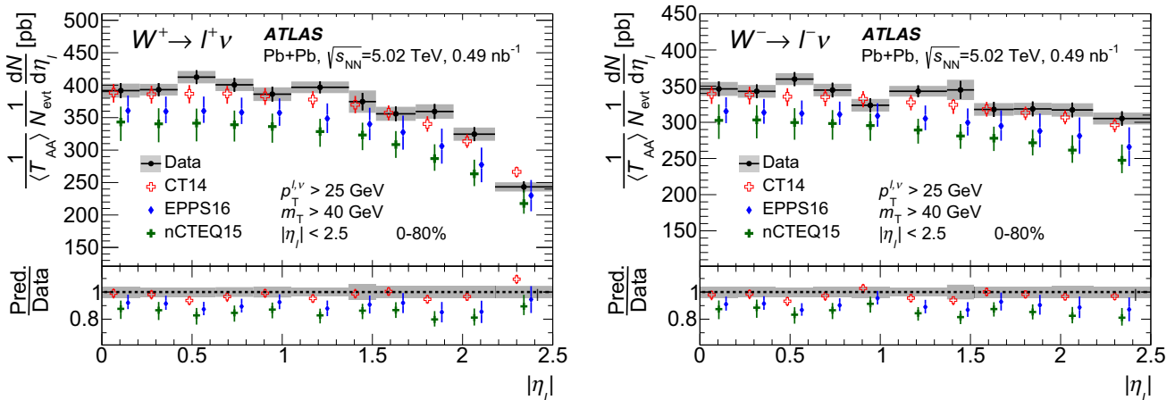
Fig. 10 Differential normalised production yields for W^+ (left) and W^- (right) bosons as a function of absolute pseudorapidity of the charged lepton for the combined electron and muon channels. Error bars show statistical uncertainties, whereas systematic uncertainties are shown as shaded boxes. Systematic uncertainties related to \langle T_{AA} \rangle are not included. The measured distributions are compared with theory predictions calculated with the CT14 NLO PDF set as well as with EPPS16
