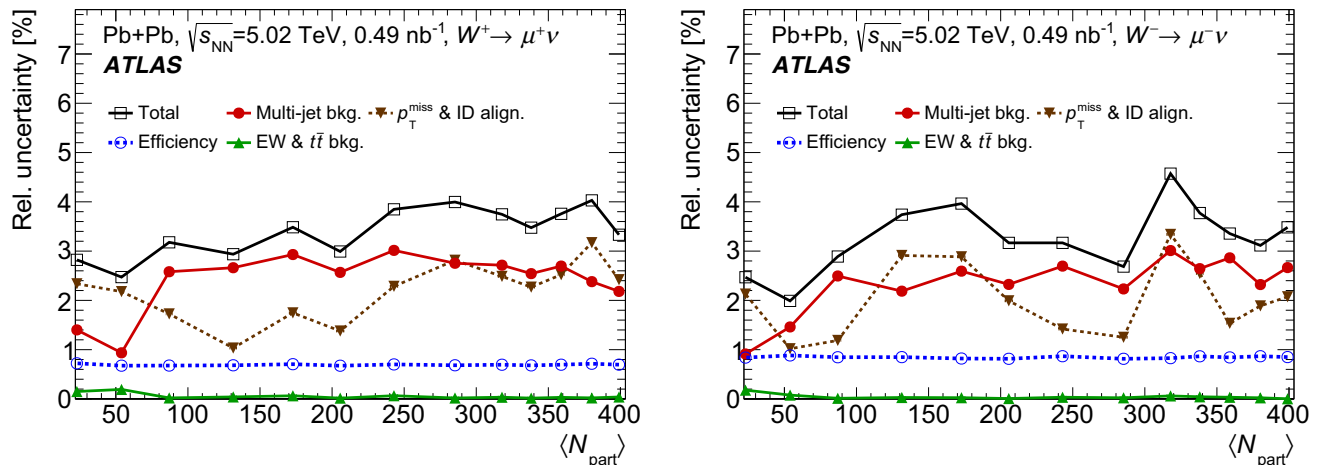
Fig. 6 Relative systematic uncertainties of W^+ (left) and W^- (right) boson production yields measured in the muon decay channel evaluated as a function of \langle N_{\text{part}} \rangle . The total systematic uncertainty is represented by open squares, while other markers represent contributions from individual sources of uncertainty. The uncertainties related to muon effi-
