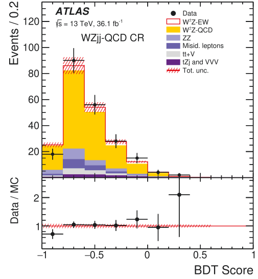
Fig. 1. Post-fit distribution of the BDT score distribution in the WZjj –QCD control region. Signal and backgrounds are normalised to the expected number of events after the fit. The uncertainty band around the MC expectation includes all systematic uncertainties as obtained from the fit.
