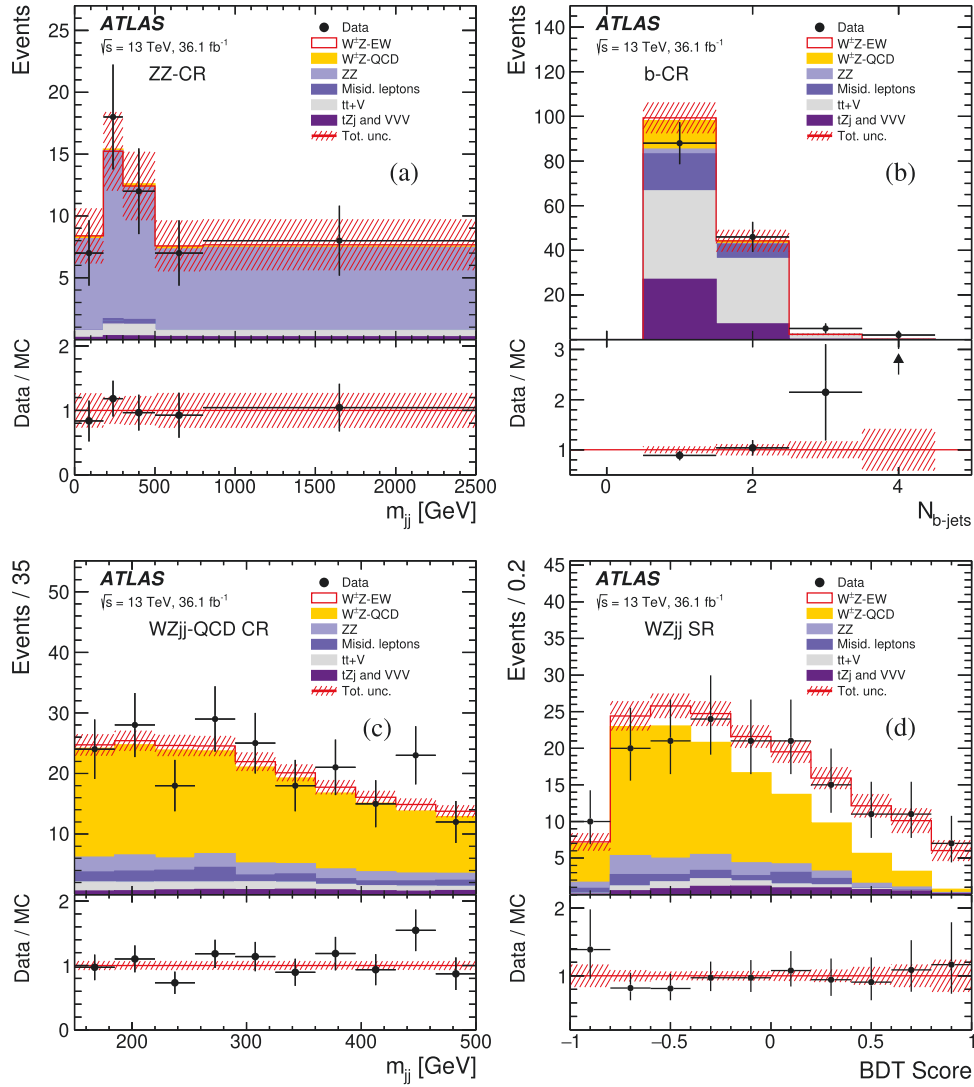
Fig. 2. Post-fit distributions of (a) m_{jj} in the ZZ-CR control region, (b) N_{b-jets} in the b -CR, (c) m_{jj} in the WZjj -QCD control region and (d) the BDT score distribution in the signal region. Signal and backgrounds are normalised to the expected number of events after the fit. The uncertainty band around the MC expectation includes all systematic uncertainties as obtained from the fit.
