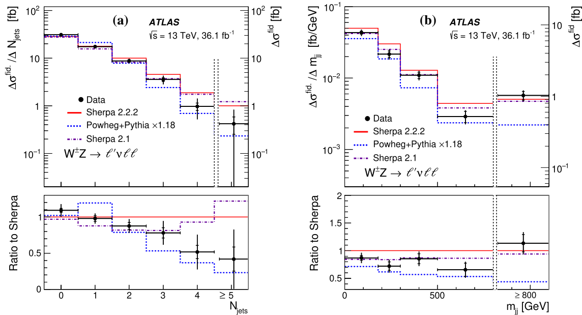
Fig. 6 The measured W^\pm Z differential cross section in the fiducial phase space as a function of the exclusive multiplicity of jets with p_T > 25 GeV (a) and of the invariant mass of the two leading jets with p_T > 25 GeV (b). The inner and outer error bars on the data points represent the statistical and total uncertainties, respectively. The measurements are compared with the predictions from SHERPA 2.2.2
