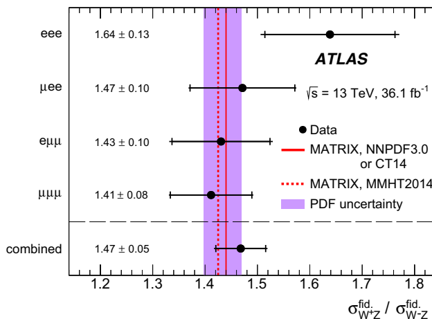
Fig. 3 Measured ratio \sigma_{W^+ Z}^{\text{fid.}}/\sigma_{W^- Z}^{\text{fid.}} of W^+ Z and W^- Z integrated cross sections in the fiducial phase space in each of the four channels and for their combination. The error bars on the data points represent the total uncertainties, which are dominated by the statistical uncertainties. The NNLO SM predictions from MATRIX using the NNPDF3.0nnlo or CT14 PDF sets are equal and represented as a single red line. The shaded violet band represents the effect of PDF uncertainties estimated using the POWHEG+PYTHIA NLO calculation using the CT10 eigenvectors and the envelope of the differences between the CT10 and CT14, MMHT2014 and NNPDF 3.0nnlo PDF sets. The MATRIX prediction using the MMHT2014 PDF set is also displayed as the dashed-red line
