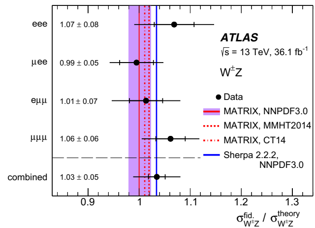
Fig. 2 Ratio of the measured W^\pm Z integrated cross sections in the fiducial phase space to the NNLO SM prediction from MATRIX in each of the four channels and for their combination. The inner and outer error bars on the data points represent the statistical and total uncertainties, respectively. The NNLO SM prediction from MATRIX using the NNPDF3.0nnlo PDF set is shown as the red line; the shaded violet band shows the effect of QCD scale uncertainties on this prediction. The prediction from MATRIX using the MMHT2014 and CT14 PDF sets and the NLO prediction from SHERPA 2.2.2 are also displayed as dashed-red, dotted-dashed-red and blue lines, respectively
