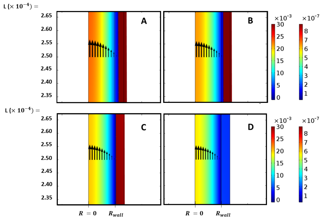
Figure 10. Animation based on Figure 9 at time ( t = 1.25 s) representing fluid-wall interplay. A, B, C and D present the corresponding Young's Modulus ( E = 3 \times 10^4, 5 \times 10^4, 1 \times 10^5, 5 \times 10^5 Pa). Total velocity and radial expansion can be seen to differ with compliance.
