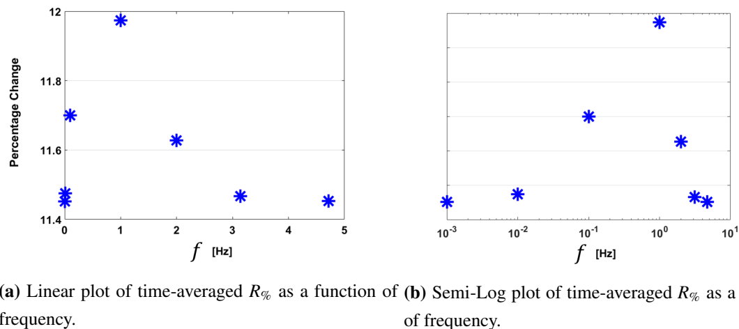
Figure 8. Plots of time-averaged R\% as a function of frequency. Resonance-type behavior is observed in the neighborhood of f = 1 Hz when assigning E = 1 \times 10^5 Pa.
