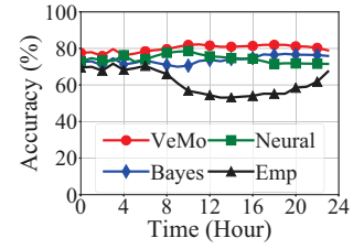
Fig 19: Route pred.
