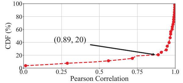
Fig 14: Speed Correlation
