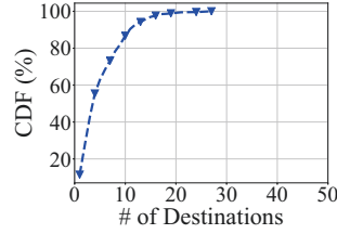
Fig 9: Crowd dest.
