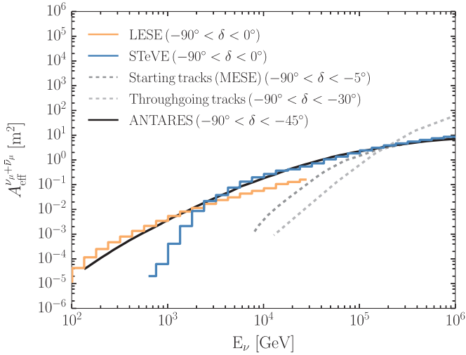
Fig. 7. Effective areas of the LESE (yellow) and STeVE (blue) selections compared to other IceCube selections using tracks: the throughgoing event selection [38] (dashed light gray) and the starting event selection (MESE) [13] (dashed gray). Also shown is the effective area for ANTARES [37] (black). The effective areas are shown for a neutrino flux \nu_\mu + \bar{\nu}_\mu and averaged over the solid angle in the declination range ( \delta ) indicated in the legend.
