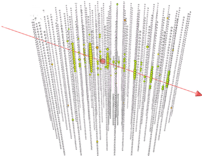
Fig. 4. An example starting event candidate of the STeVE selection.
