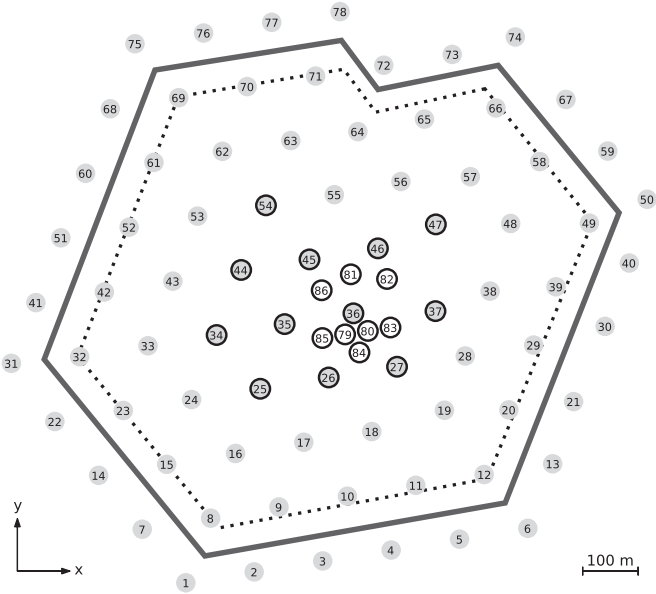
Fig. 1. Top view of the IceCube detector with dots representing the positions of the numbered sensor strings. While gray dots indicate strings with nominal string spacing, white dots with a black border indicate strings with a higher DOM density, forming a low-energy extension of IceCube called DeepCore. The strings marked with a black border are used to form one of the primary IceCube triggers as explained in the main text. The polygons define different volumes which are used in the FSS filter (solid grey) and the STeVE and LESE event selections (dashed grey) described in Section 3 and 4, respectively.
