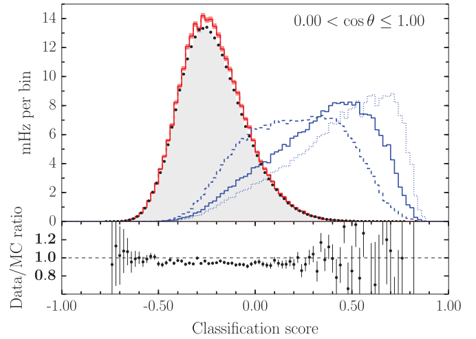
Fig. 6. Classification score for the LESE selection. Experimental data is shown in black dots and illustrated by a gray shaded area. The total background simulation including both atmospheric muons \mu and atmospheric muon-neutrinos \nu_\mu are shown using a red solid line, with a red shaded area indicating the statistical uncertainty. Different signal hypotheses are displayed in blue lines: E^{-3} (dashed), E^{-2} e^{-E_\nu/10\text{TeV}} (solid), and E^{-2} (dotted), each normalized to the event rate in experimental data. The bottom panel shows a comparison between experimental data and the total background simulation. Figure adapted from [15].
