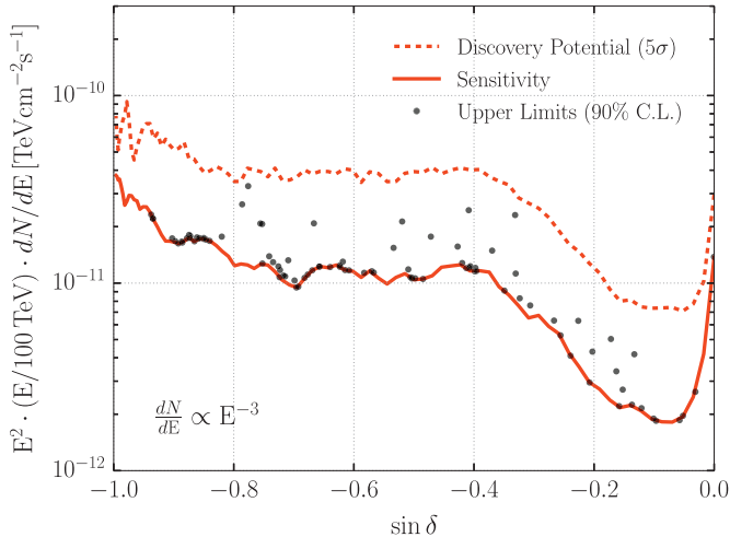
Fig. 12. Sensitivity and 5\sigma discovery potential as functions of declination, with flux upper limits for each object in the source catalog assuming a soft spectrum ( \gamma = 3 ).
