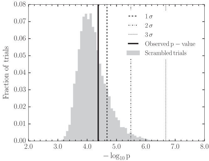
Fig. 11. Distribution of the most significant p -value from the southern sky search, obtained from 10,000 randomized trials with scrambled data. The dashed vertical lines represent the 1, 2, and 3 \sigma limits. The most significant p -value observed is indicated with a solid vertical line.
