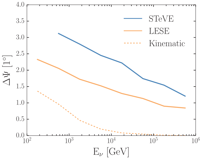
Fig. 8. Median angular resolution for the LESE (yellow) and STeVE (blue) selections. Also shown is the kinematic angle for the LESE selection (yellow dashed). The latter is defined as the angle between the neutrino-induced muons and the corresponding primary neutrinos and illustrates the limit to our resolution for this event selection.
