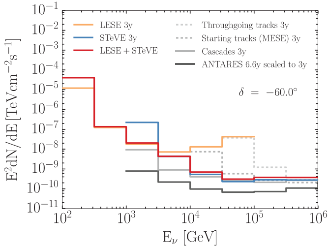
Fig. 9. The differential discovery potential at -60^\circ declination for LESE (yellow), STeVE (blue), the combined selection (LESE+STeVE) (red), a cascade point-source search [8] (gray), a starting tracks search targeting higher energies (MESE) [13] (gray dashed), throughgoing [38] (light gray dashed), all with the IceCube detector, and of the point-like source search with the ANTARES detector [42] based on the analysis in [37] (black). In this plot, all results are calculated for an equal three year exposure.
