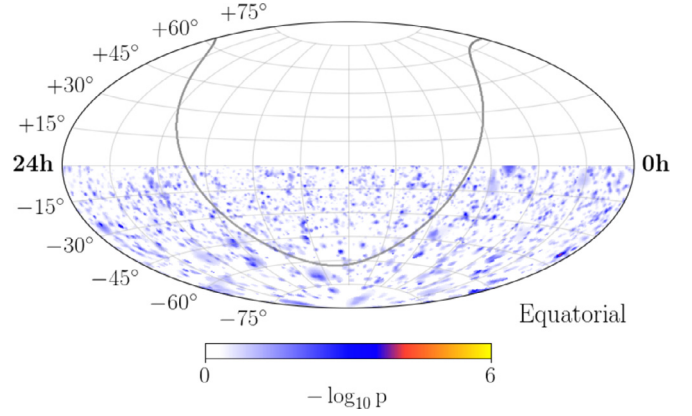
Fig. 10. Pre-trial significance map in equatorial coordinates (J2000). The black line indicates the Galactic plane.
