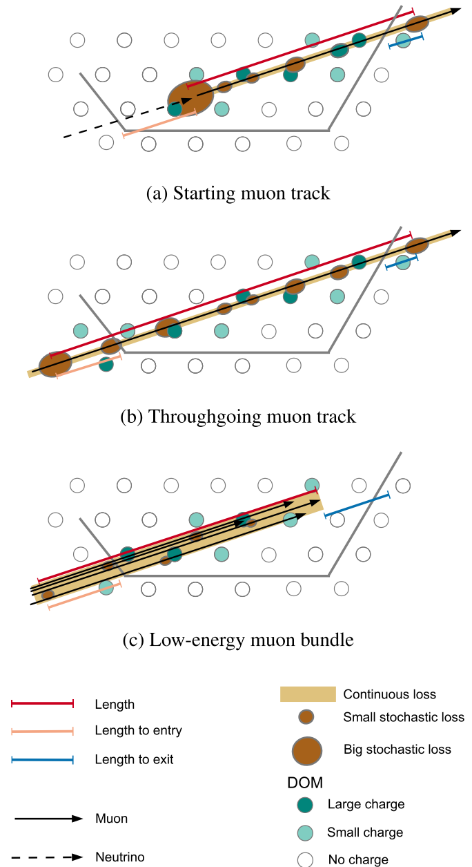
Fig. 3. Top view of different track-like events in the IceCube detector, showing quasi-continuous and stochastic energy losses as well as the definition of three useful track length variables. Figure adapted from [14].
