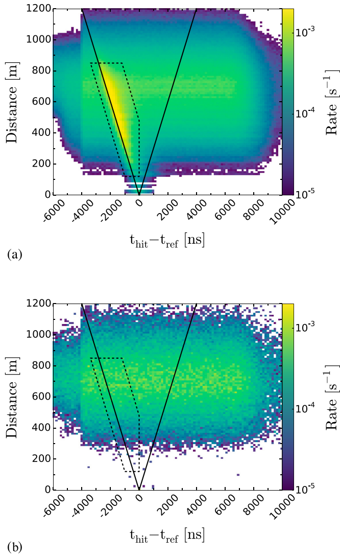
Fig. 5. Distance in space and time between SLC hits in the top veto region and the first HLC hit in the fiducial volume. The two solid black lines converging at the position of the reference hit (0,0), illustrate the light-cone. The color (z-axis) indicates the event rate. (a) Experimental data. (b) Simulated, truly down-going, muon neutrinos interacting inside the volume defined by the dotted polygon in Fig. 1 and z \leq 300 m.
