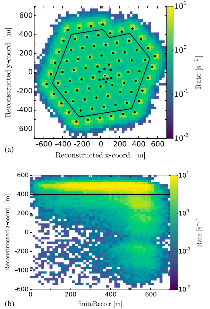
Fig. 2. Distributions of reconstructed interaction vertices for experimental data before the application of the FSS filter. The color (z-axis) indicates the event rate. (a) Top view of the IceCube detector where string positions are shown as black dots. The polygon shape represents the containment criterion for the reconstructed interaction vertices (see also Fig. 1). (b) Side view of the detector where the horizontal black line indicates the containment criterion used in the top veto of the FSS filter. The horizontal axis (“reconstructed r ”) shows the position of the vertex in the xy -plane, i.e. \sqrt{x^2 + y^2} . Note that z = 0 corresponds to the center of the detector.
