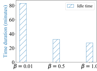
Fig. 12: Impact of \beta on idle time
