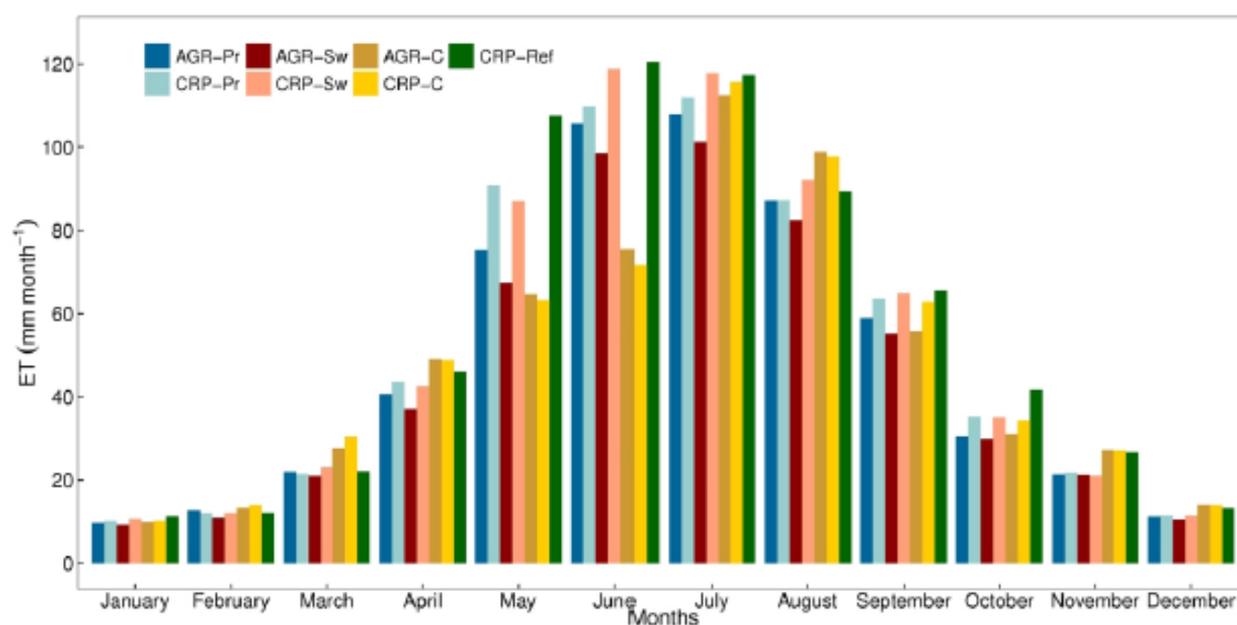
Fig. 7. Average monthly evapotranspiration (ET) rates from 2013 to 2017 for each field. See Fig. 1 for land use conversion history and site names.
