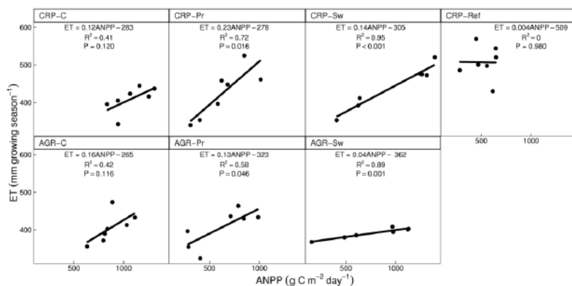
Fig. 2. Mean aboveground net primary productivity (ANPP, n = 10 ) vs. growing season (May–Sept) evapotranspiration ( ET_{gs} ) for all fields from 2010 through 2016. ANPP for the corn fields does not include seeds. See Fig. 1 for land use history and field names.
