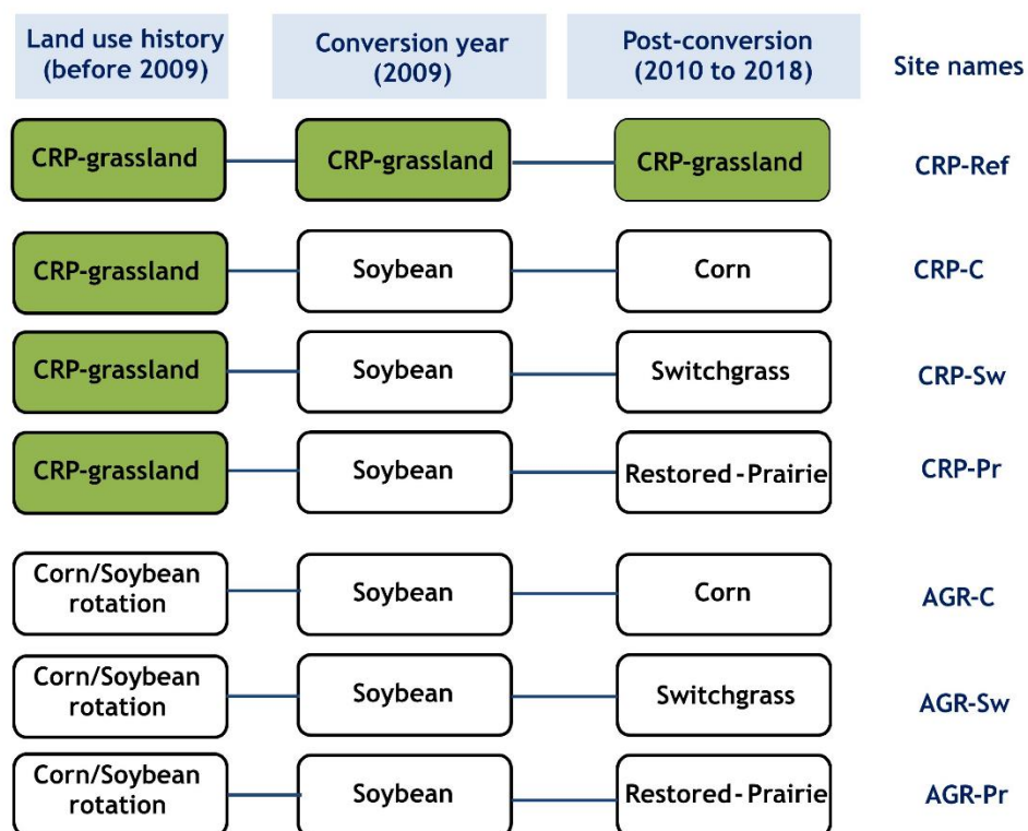
Fig. 1. A schematic illustration of land use history and conversion at study sites. Fields were converted from Conservation Reserve Program (CRP) grasslands and conventionally tilled corn-soybean rotation agricultural (AGR) fields. The CRP grasslands were under smooth brome grass since 1987 and the AGR in row crops at least for 5 decades prior to conversion in 2009. Fields were first converted to no-till soybean in 2009, then to no-till corn (C), switchgrass (Sw) or restored prairie (Pr) from 2010 onward. The CRP-Ref was maintained in smooth brome grass that was not harvested.
