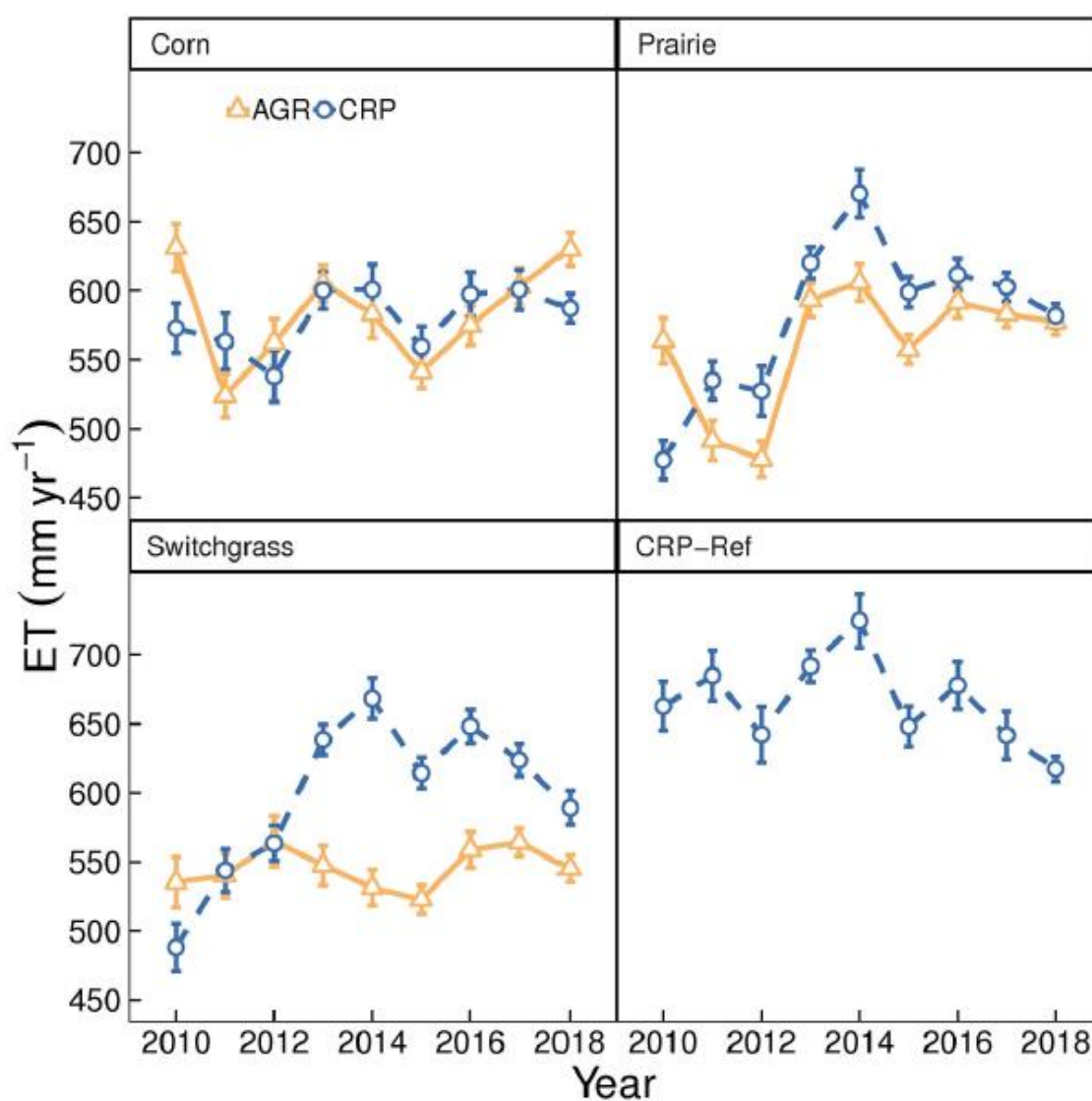
Fig. 6. Annual evapotranspiration ( ET_t ) rates from 2010 through 2018 for all fields. Annual ET includes data from October of the previous year to September of the current year. See Fig. 1 for land use conversion history.
