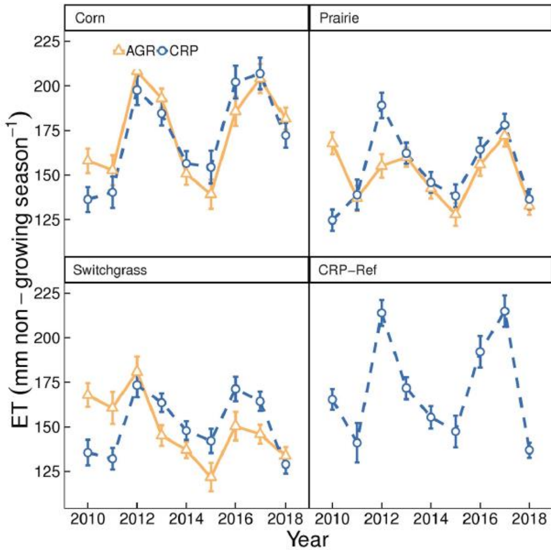
Fig. 5. Non-growing season evapotranspiration (ET ngs ) rates from 2010 through 2018 for all fields.
