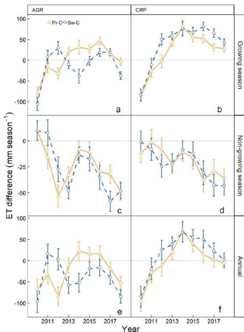
Fig. 3. Growing season, non-growing season and annual evapotranspiration (ET) differences between the perennial (restored prairie and switchgrass) crops and corn from 2010 through 2018. The legend Pr-C refers to restored prairie ET less corn ET, and Sw-C refers to switchgrass ET less corn ET. The growing season is May to September, the non-growing season is from October of previous year to April of current year, and annual spans October of previous year to September of current year. Error bars – representing uncertainty – that lie along the broken horizontal line indicate similar ET between the perennials and corn, points above the line indicate ET rates for perennials higher than those for corn while those below the line indicate ET rates for perennials less than those for corn. See Fig. 1 for land use conversion details.
