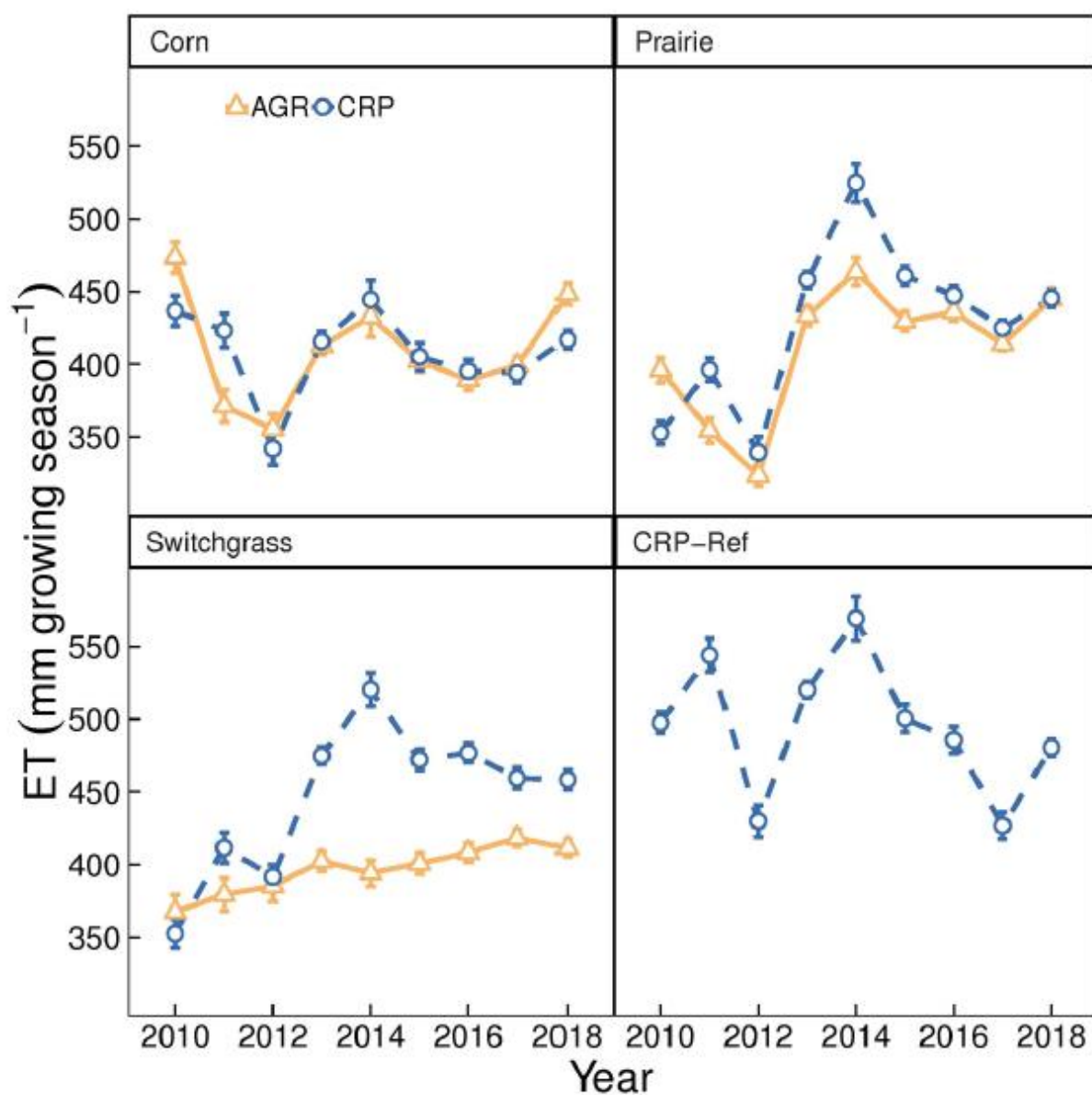
Fig. 4. Growing season (May–Sept) evapotranspiration (ET gs ) rates from 2010 through 2018 for all fields. See Fig. 1 for land use conversion history.
