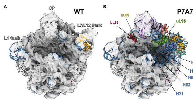
Figure 2. Comparison of (A) WT 50S and (B) P7A7 large subunit cryo-EM maps. Maps are low-pass-filtered to 8 Å for clarity of structural features, and 50S coordinates from PDB 4YBB 44 are docked to identify missing components. The central protuberance (CP), L1 Stalk, and L7/L12 Stalk are identified on the WT structure, and features confirmed to be missing from P7A7 by combined cryo-EM and LC-MS/MS analysis are labeled on the P7A7 structure.
