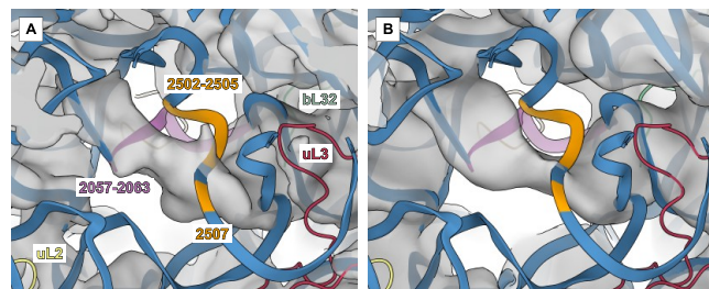
Figure 6. Comparison of (A) PTC in the P7A7 map and (B) an assembly intermediate, E4, determined by Davis et al. 46 Both maps show helical density that does not appear in fully assembled WT structures. P7A7 mutations regions 2057–2063, and 2502–2505 and 2507, are colored in pink and orange, respectively. Other 23S rRNA regions are shown in blue, and nearby proteins uL2, uL3, and bL32 are shown in yellow, red, and green, respectively.
