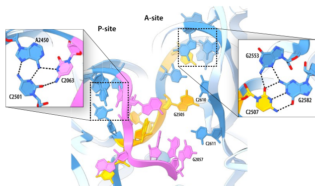
Figure 5. WT 23S rRNA residues directly affected by P7A7 mutations. Coordinates shown are from PDB 4YBB. 44 Mutated residues 2057–2063, and 2502–2505 and 2507, in P7A7 are depicted in pink and gold, respectively. Unaltered bases within 3 Å of mutations are shown in darker blue, and those further away are lighter blue. Close-ups highlight base triples that would be disrupted by mutations, and two disrupted base pairs are also labeled.
