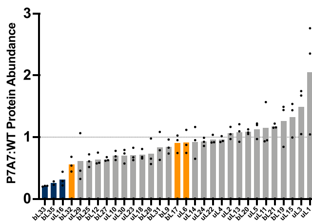
Figure 3. 50S ribosomal protein ratios detected by LC-MS/MS and TMT relative quantitation between P7A7 and WT ribosomes. Bars represent means and are colored based on the absence in final assembly states (E4 and E5) of Davis and Tan et al. (orange) or the absence in both Davis et al. 46 and Nikolay et al. 57 states (IV and V) (blue).
