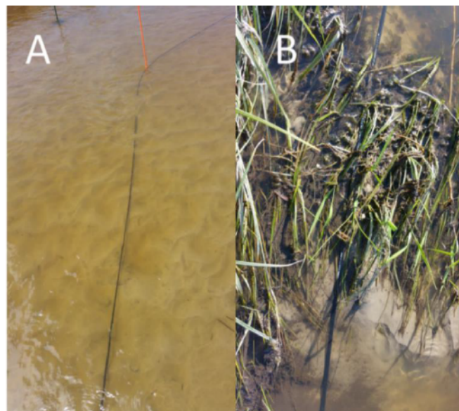
Figure 2. (A) Fiber-optic cable deployed on the streambed and (B) an example of a case where the cable was occasionally above the water surface either due to difficulty in deploying the cable or a bunch in the channel due to a slight decrease in stage during the study period.
