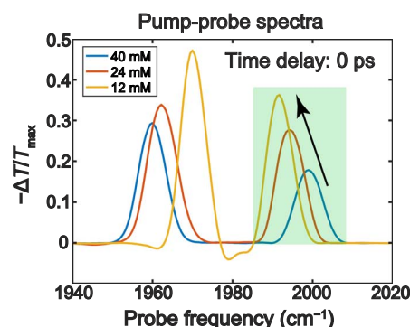
Fig. 2. Polariton bleach effect at a pump-probe delay time ( t_2 ) of 0 ps (optical nonlinearity) as a function of concentration. From the pump-probe spectra, the bleach signal (normalized to the maximal linear transmission peak intensity) increases as the molecular concentration decreases.
