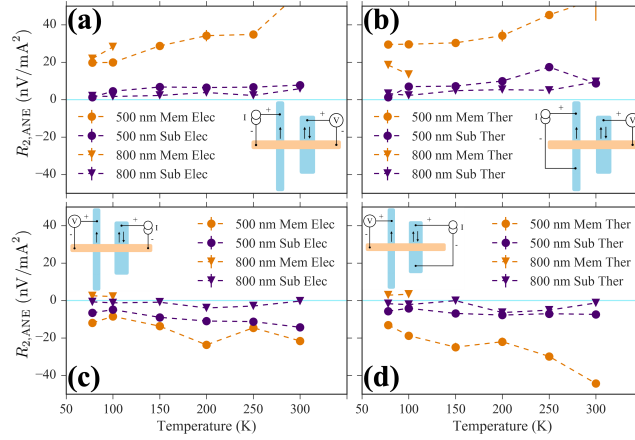
FIG. 8. R_{2,ANE} vs. T for L = 500 nm and L = 800 nm membrane- and substrate-supported devices in electrical (a,c) and thermal (b,d) spin injections for Orientation A (a,b) and Orientation B (c,d).
