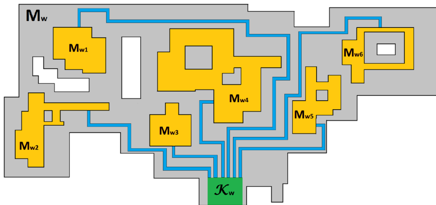
Fig. 3 The subtree of \mathcal{S} inside M_w
