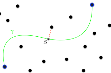
Figure 1: In this figure we have a collection of points. The length or cost of the green curve between the two blue points is the integral along the curve scaled by the distance to the nearest point.
