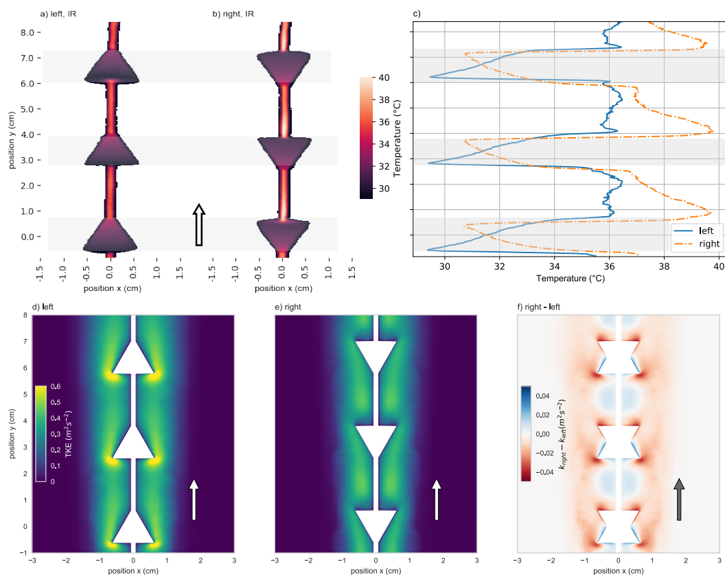
Figure 5. The brightness temperature of the fiber-optic cables with (a) left and (b) right pointing cones for the 12mm, 1:1 cones with 2cm spacing and a heating rate of 2.5 \text{ W m}^{-1} for a wind speed of 0.9 \text{ m s}^{-1} . (c) The average of the three warmest pixels in each horizontal row is provided to better demonstrate the spatial pattern of temperatures along the fiber. The grey shading is to visually line up the cones in a-c. (d, e) Turbulence kinetic energy (TKE) computed from the CFD simulations for the same experiment as in (a) and (b) with (f) the difference in TKE between the two orientations. The difference in TKE was not physically meaningful in the region with a cone in either (d) or (e) and is excluded in (f). The subset arrows indicate the direction of the mean flow.
