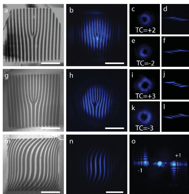
Figure 4. Generation of SH vortices with \text{TC} = 2, 3 , and Airy beam. (a) SEM image and (b) SH image of the fabricated CGH on \text{WS}_2 monolayer for generating SH vortex with \text{TC} = \pm 2 . (c,e) Far-field images of SH vortices in the +1 and −1 diffraction order and (d,f) the corresponding cylindrical lens images indicating the TC of +2 and −2, respectively. (g–l) Experimental results for generating SH vortex with \text{TC} = \pm 3 . (m) SEM image of the fabricated CGH with cubic phase modulation on \text{WS}_2 monolayer for producing the 2D-Airy beam. (n) SH image of the same hologram. (o) Far-field image of SH Airy beams at the \pm 1 diffraction order. Scale bars are 10 \mu\text{m} .
