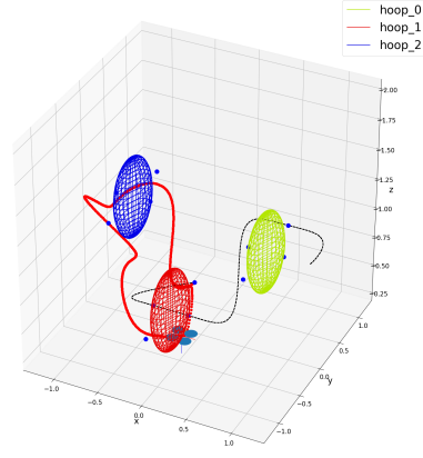
Fig. 5. A satisfying run from the LTL specification ( \phi = \square(\Diamond hoop_0 \rightarrow \neg hoop_1 \cup hoop_2 \wedge \Diamond hoop_1) ). We show the prefix portion of the trajectory in black and the suffix portion in red. The suffix portion indicates the set of hoops that can be visited infinitely often.
