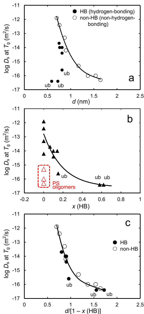
FIG. 1. Surface diffusion coefficient D_s at T_g plotted as a function of (a) d , (b) x(\text{HB}) , and (c) d/[1-x(\text{HB})] . "ub" stands for "upper bound" (see Table II). The curves are guide to the eye.
