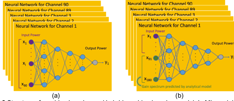
Fig. 2 Structure of machine learning and hybrid machine learning model. In ML model, 90 features ( x_1-x_{90} ) of input channel power are used and 4 hidden layers have 90 neurons each. The output is the optical channel power. In HML model, 90 features ( x_1-x_{90} ) of input channel power and another 90 features ( x_{91}-x_{180} ) of gain spectrum predicted by analytical model are used. The hidden layers have 180, 90, 90, 45 neurons.
