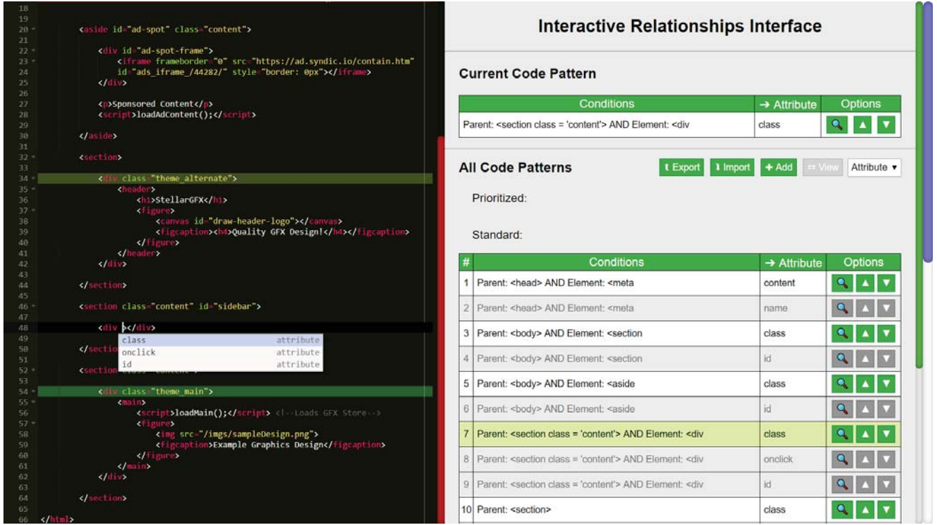
Fig. 1. As developers type in the HTML editor (left side), the autocomplete menu is displayed to offer suggested code completions. In the IRIS interface (right side), the Current Code Pattern explains to the developer the basis for the first suggested completion.
