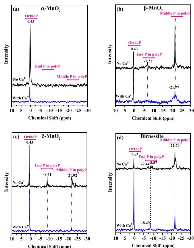
Figure 3. ^{31}\text{P} solution NMR spectra of liquid supernatants obtained after polyphosphate ( \text{P}_{10} ) reaction with \alpha\text{-MnO}_2 (a), \beta\text{-MnO}_2 (b), \delta\text{-MnO}_2 (c), and birnessite (d) at pH 6.0 with or without 500 \mu\text{M} \text{Ca}^{2+} for 5 d.
