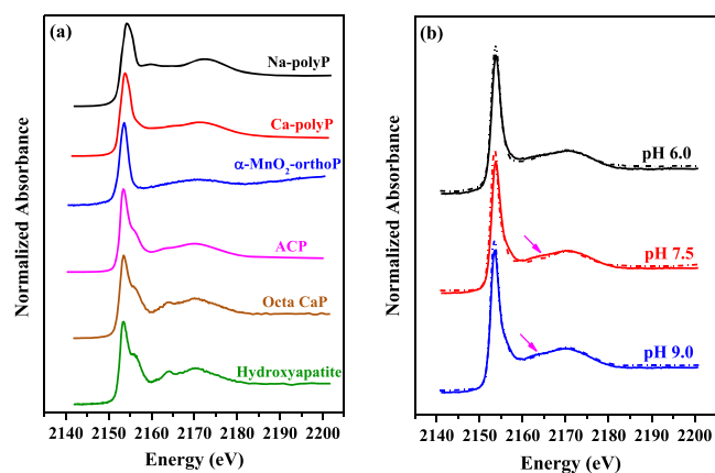
Figure 8. (a) P K-edge XANES spectra of phosphate reference compounds, including sodium polyphosphate salt (Na-polyP), synthesized calcium polyphosphate granules (Ca-polyP), \alpha - \text{MnO}_2 adsorbed orthophosphate ( \alpha - \text{MnO}_2 -orthoP), amorphous calcium phosphate (ACP), octacalcium phosphate (octaCaP), and hydroxyapatite. (b) Linear combination fitting of P XANES spectra of the solid reaction products from the hydrolysis experiments of Ca-polyP with \alpha - \text{MnO}_2 at pH 6–9. Reaction condition: \alpha - \text{MnO}_2 = 0.4 \text{ g L}^{-1} ; Ca-polyP granule = 0.02 \text{ g L}^{-1} ; NaCl = 0.1 \text{ M} . Raw and fitted data are shown in dotted and solid lines, respectively. Fitting results are presented in Table S2.
