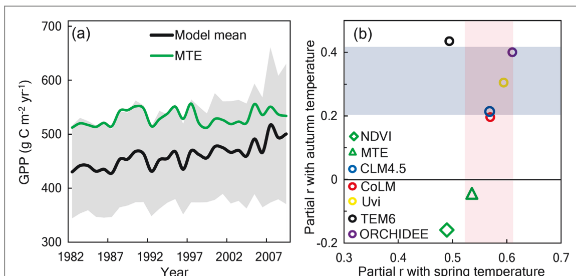
Figure 4. Temporal variations of GPP and its dependence on spring and autumn temperature. (a) Temporal changes of annual total GPP over northern lands ( >50^{\circ} N) from a flux-based dataset (i.e. MTE) and five terrestrial biosphere models (see methods). The green line show the annual MTE GPP. The black line represents the model averages and the gray area is the standard deviation among models. (b) Mean partial correlation coefficient (partial r ) of NDVI and GPP to spring temperature and autumn temperature changes. The shaded areas represent the standard deviations of the partial r among models. Note that only the grid cells with significant partial correlation ( P < 0.05 ) were included in this analysis.
