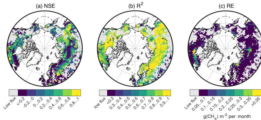
Figure 8. NSE, R^2 and RE calculated between RF-DYPTOP and LPX-Bern. Grid cells with low CH 4 wetland emissions (below 0.1 \text{ g}(\text{CH}_4) \text{ m}^{-2} \text{ yr}^{-1} ) are shown in grey. RE values refer to total unit area in a grid cell.
