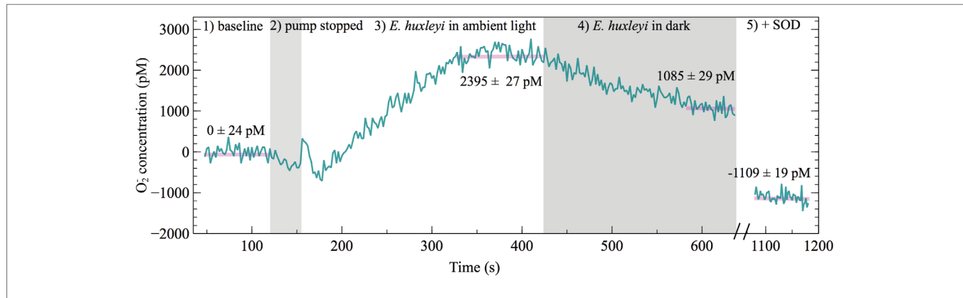
FIGURE 6 | FeLume time-series of O_2^- measurements under different light conditions on day 2 of E. huxleyi growth (biological replicate B) split into five regions: (1) phosphate buffer solution and MCLA reagent baseline (which is subtracted from the biogenic O_2^- concentration in regions 3 and 4), (2) shaded region showing loading of E. huxleyi cells while the pump was stopped, (3) E. huxleyi in ambient light, (4) the second shaded region showing E. huxleyi in the dark, and (5) drawdown of the O_2^- signal below the baseline after addition of SOD (negative O_2^- concentrations account for SOD driven degradation of O_2^- originating from auto-oxidation of the MCLA reagent). The average \pm SE of stable steady-state O_2^- concentration measurements are indicated by horizontal pink lines.
