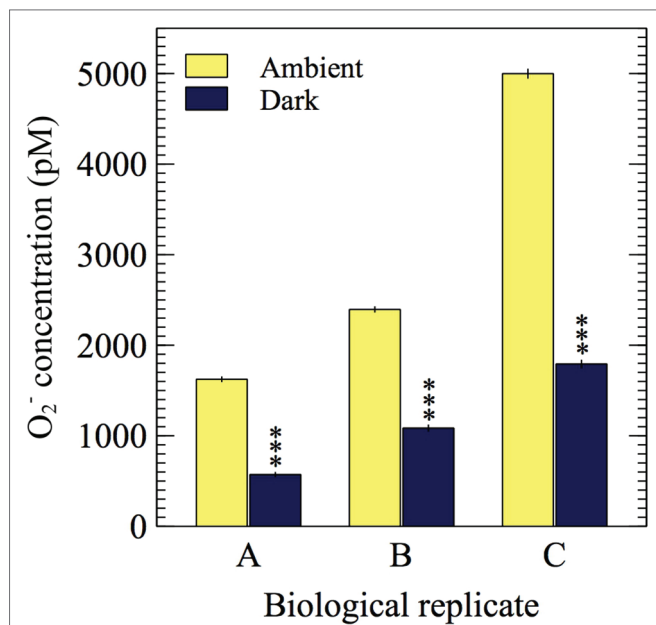
FIGURE 7 | O_2^- measurements from three biological replicates of E. huxleyi in the presence of ambient light ( \sim 5 \mu\text{mol photons m}^{-2} \text{s}^{-1} ) and in the dark ( 0 \mu\text{mol photons m}^{-2} \text{s}^{-1} ). Asterisks show significant difference ( p < 0.0001 ) between the average dark and average ambient light steady-state O_2^- concentration for each biological replicate. Error bars represent one standard error of the mean ( n \geq 31 chemiluminescent counts).
