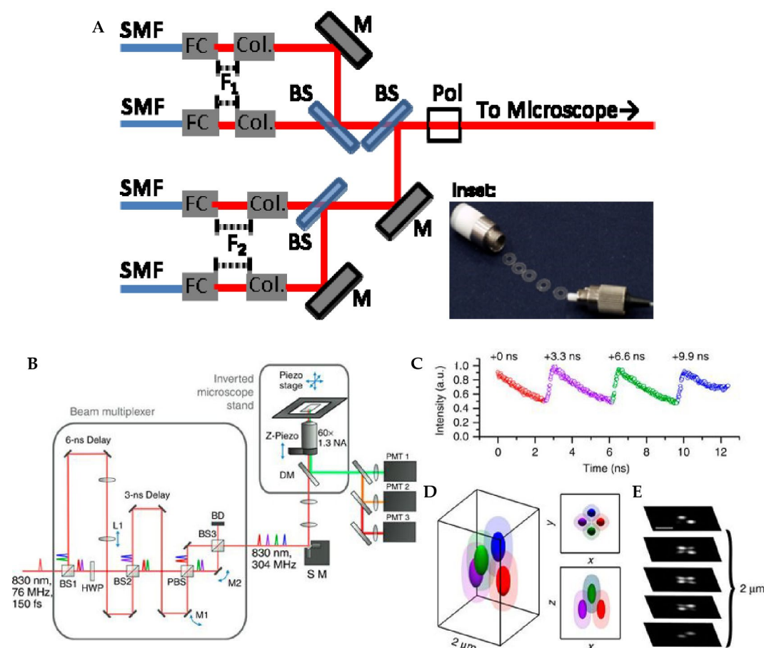
Figure 9. (a) Schematic of tetrahedral excitation tracking setup, where four laser diode beams are combined by 3 beam splitters and focused onto the sample in a tetrahedral pattern. (inset) Washers inserted between the fiber coupler (FC) and collimator (Col) are used to arrange the four laser foci after the objective. Adapted from reference [92]. Copyright 2015 Optical Society of America. (b) Schematic of TSUNAMI. A pulsed laser is split by two beam splitters to generate four laser beams. The temporal separation between four beams is achieved by physical delay. The arrangement of the four foci after the objective is controlled by mirrors in the excitation beam path. (c) Temporal separation of the four excitation beams measured by the fluorescence of an emitter in the center of the detection volume. (d) Schematic of the tetrahedral PSF. (e) Scanning image of 100 nm fluorescent beads in different depth. Scale bar: 2 \mu\text{m} . Adapted from reference [93] under Creative Commons Attribution 4.0 International License.
