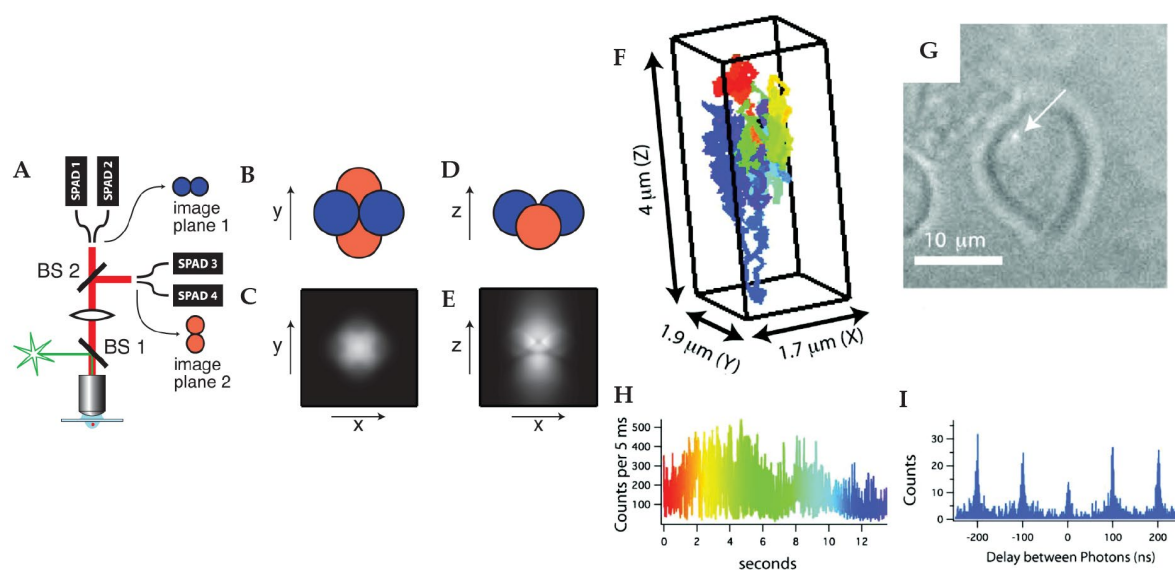
Figure 4. Tetrahedral detection active feedback 3D tracking. (a) Schematic of experimental setup. BS: beamsplitter; SPAD: single-photon counting avalanche photodiode. (b, d) Schematic of the sample volume viewed along Z (b) and Y (d) axis, in which the four balls represent the sample volumes of four SPC-APDs. (c, e) Total fluorescent intensity in the Z=0 plane (c) and Y=0 plane (e). Reprinted from reference [68], with the permission of AIP Publishing. (f) 3D trajectory of a single quantum dot labeled high-affinity immunoglobulin E receptor (IgE-FcεR) in a live cell. The rainbow color from red to blue indicates time. (g) Image of cell and the actively tracked receptor (white arrow). (h) Fluorescence intensity of the quantum dot probe as a function of time. (i) Photon pair correlation measurement shows fluorescence photon antibunching, indicating a single quantum emitter. Reprinted with permission from reference [71]. Copyright 2010 American Chemical Society.
