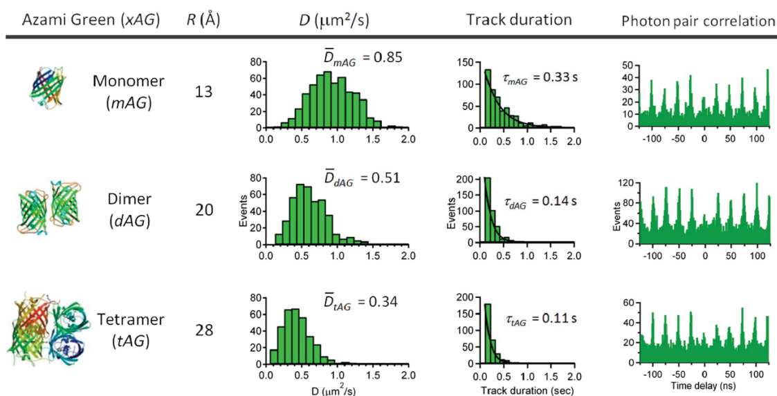
Figure 16. RT-3D-SMT using the tetrahedral detection method reveals the protein oligomerization states of Azami Green oligomers mAG, dAG, and tAG in 92% glycerol solution. Reprinted with permission from reference [106]. Copyright 2012 American Chemical Society.
