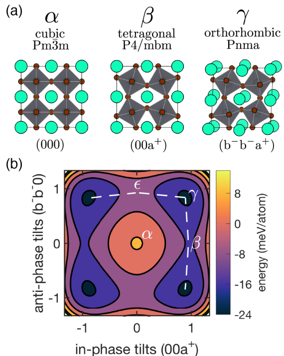
FIG. 1. (a) Many halide perovskites such as \text{CsPbBr}_3 undergo a series of structural transitions upon cooling, starting in a cubic form at high temperature and transforming to tetragonal and orthorhombic forms at low temperature as a result of octahedral tilts. (b) The energy surface of \text{CsPbBr}_3 as a function of octahedral tilts, calculated with density functional theory for configurations with orthorhombic lattice parameters. For each configuration, the \text{PbBr}_6 sublattice and lattice parameters were held fixed while the Cs sublattice was allowed to relax. The energy surface shows that the cubic phase, \alpha , coincides with a local maximum, the tetragonal phase, \beta , resides at a saddle point, and the ground state orthorhombic phase, \gamma , corresponds to a stable minimum. (Crystal structures visualized using the VESTA program suite [50])
