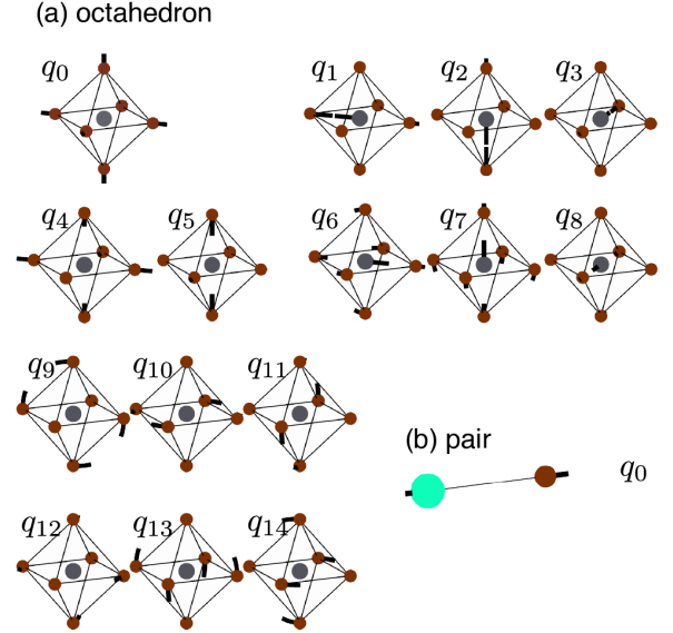
FIG. 3. Collective cluster deformations (CCDs) for (a) an octahedron and (b) a pair. The octahedral CCDs are organized by irreducible representations, with one 1D irrep, one 2D irrep and four 3D irreps. A pair cluster has only one CCD corresponding to the pair distance.
