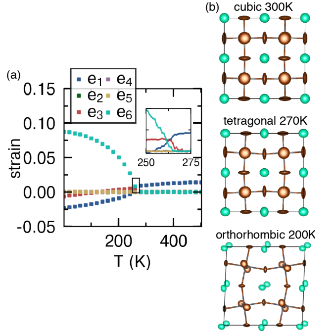
FIG. 6. (a) Thermodynamically averaged strain order parameters as calculated with Monte Carlo simulations applied to the anharmonic cluster expansion of Table I. (b) Thermodynamically averaged displacement covariances were used to compute the atomic displacement parameters (ADP). The ADP ellipsoids enclose 90% of the cumulative probability density of atomic motion.
