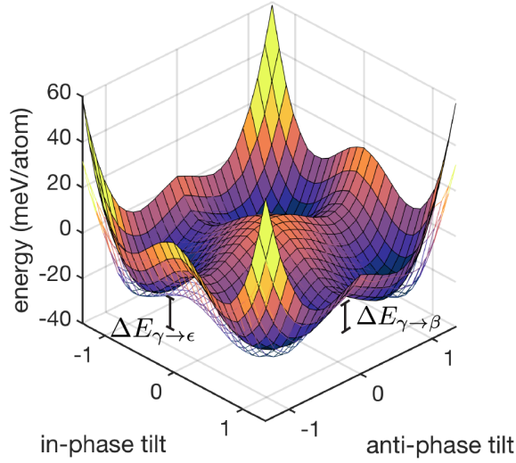
FIG. 5. Linearized model energy landscape (surface) compared to the DFT energy landscape (mesh). Energy barriers through the \epsilon -phase and \beta -phases are depicted and labeled \Delta E_{\gamma \rightarrow \epsilon} and \Delta E_{\gamma \rightarrow \beta} respectively. The linear model reproduces many of the qualitative features of the DFT energy landscape; however it overestimates the energy barrier \Delta E_{\gamma \rightarrow \epsilon} .
