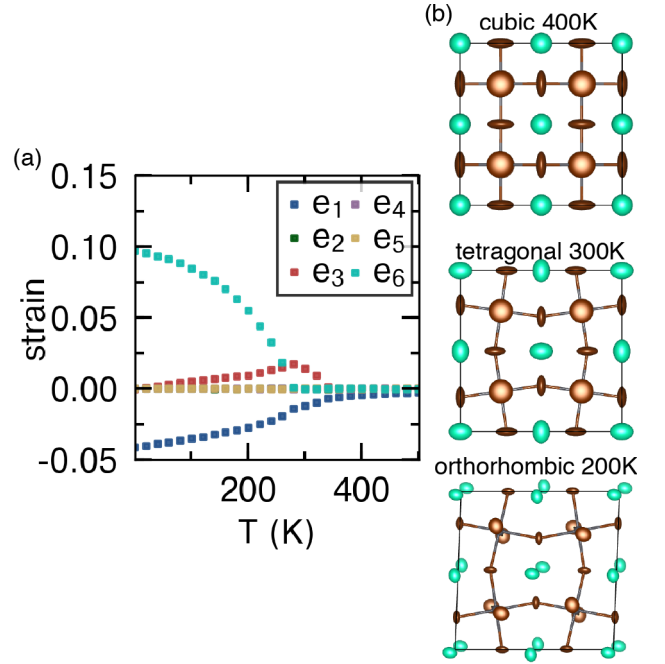
FIG. 8. (a) Thermodynamically averaged strain order parameters from Monte Carlo simulations using an anharmonic vibrational Hamiltonian that stabilizes the \beta phase over a wide temperature interval (see text for more details). Representative structures are shown in (b), along with thermodynamically averaged ADP ellipsoids, which enclose 90% of the cumulative probability density of atomic motion.
