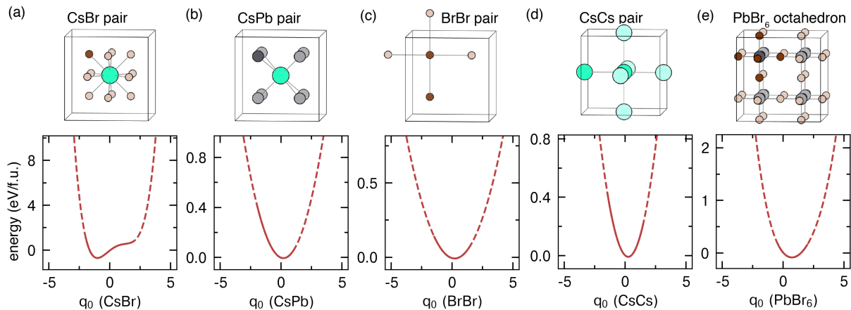
FIG. 4. (a-e) Symmetrically equivalent clusters (top panel) and evaluated cluster energy function (bottom panel) as a function of q_0 (volumetric deformation) for each cluster included in the anharmonic vibrational Hamiltonian.
