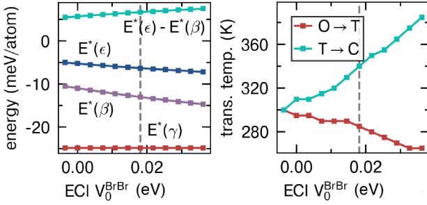
FIG. 7. (a) Energies of \gamma , \beta and \epsilon relative to undistorted \alpha (set equal to zero) as a function of V_0^{\text{BrBr}} while keeping the relative values of all other coefficients of the anharmonic vibrational Hamiltonian of Table I constant (all Hamiltonian coefficients were rescaled to maintain a constant difference in energy between \gamma and \alpha ). (b) Transition temperatures as a function of V_0^{\text{BrBr}} . The temperature interval in which the tetragonal \beta phase is stable increases as the energies of \beta and \epsilon decrease relative to that of \gamma . The dashed gray line indicates an ECI value of 0.018 eV and is the model used to investigate local octahedral tilt environments.
