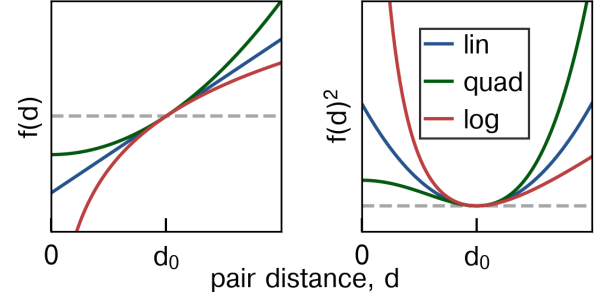
FIG. 2. (a) Linear (blue), quadratic (green), and logarithmic (red) pair functions plotted as a function of pair distance. The reference pair distance is denoted as d_0 and the dotted line represents f(d) = 0 . (b) The square of the different pair functions are plotted. The log function is used in this study in order to penalize pair contraction over pair expansion giving rise to volumetric expansion upon heating.
