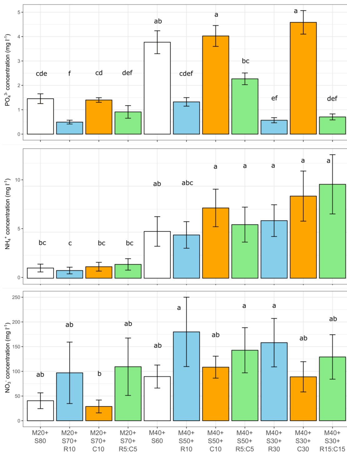
Figure 5. Mean ± SEM leachate nutrient concentrations among different treatments containing varying volumes of compost (“M”), WTR (spent lime; “R”), coir (“C”) and WTR: coir mixture in laboratory bioretention columns. Ratios of each of the substrates are indicated next to the letters. Varying letters indicate significant differences among treatments ( p < 0.05 ). Bars in white= no WTR or coir, blue = WTR, orange= coir, green= WTR: coir mix.
