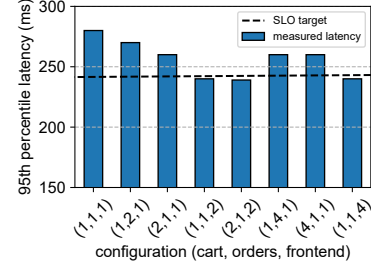
(b) Tail latency of orders workflow for various resource scaling configurations. The configuration suggested by the optimization of CPU utilization thresholds is (1,1,2) i.e one pod for cart, one pod for orders and two pods for frontend. All other microservices are provisioned with one pod.
