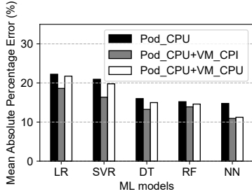
(a) Mean absolute percentage error.
