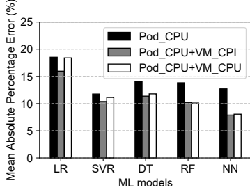
(a) Mean absolute percentage error.
