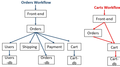
Fig. 2: Workflow DAGs.
