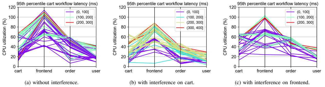
Fig. 5: Impact of performance interference on multivariate relationship between CPU utilization and end-to-end tail latency of cart workflow.
