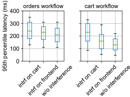
Fig. 6: Impact of performance interference on the end-to-end tail latency of various workflows.
