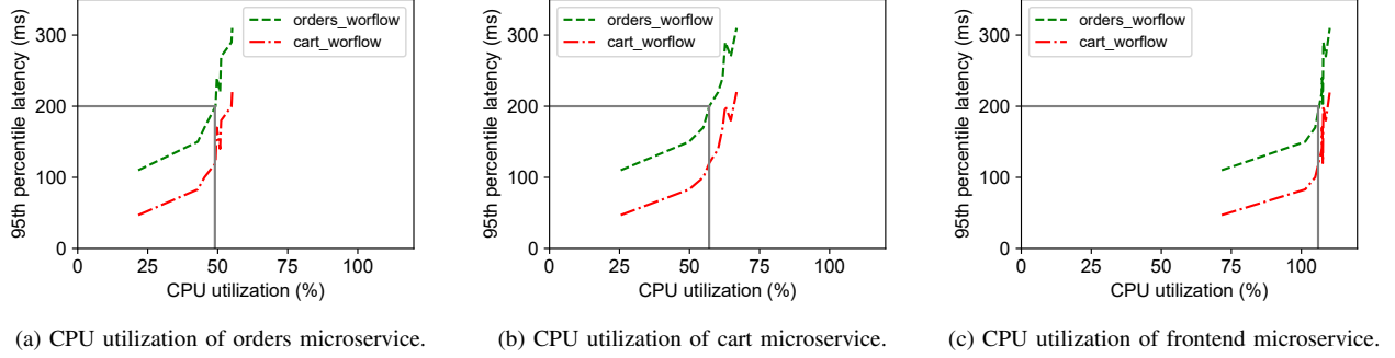
Fig. 3: Impact of CPU utilization on the tail latency of various workflows.
