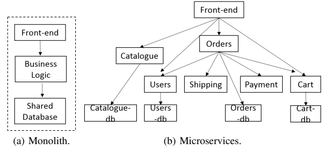
Fig. 1: Monolithic vs microservice architecture.
