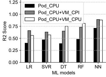
(b) R^2 Score.
