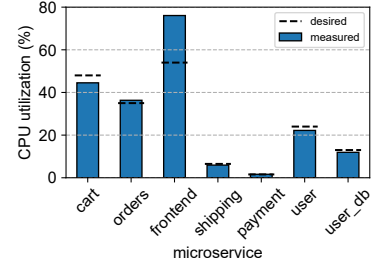
(a) Current vs desired average CPU utilization of various microservices. Here, one pod is allocated to each microservice.
