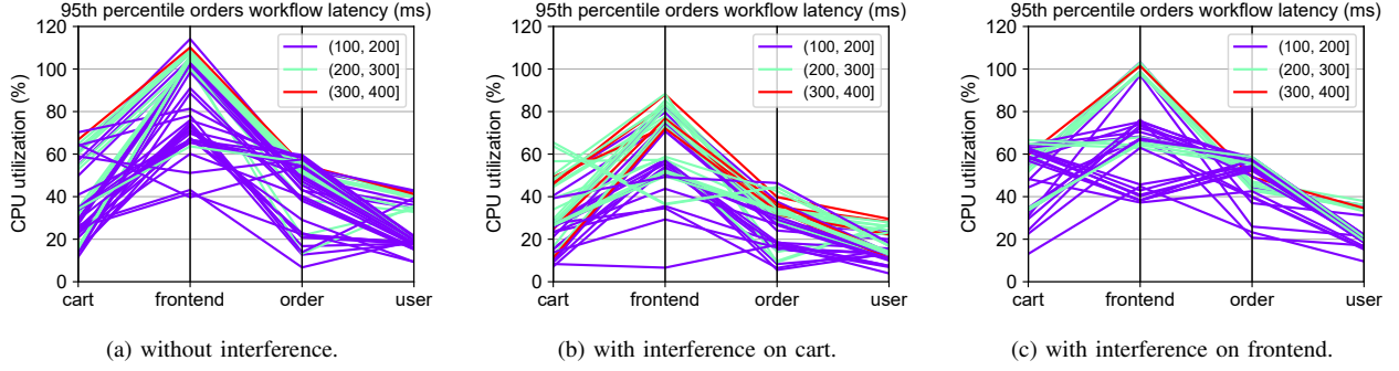
Fig. 4: Impact of performance interference on the multivariate relationship between CPU utilization and end-to-end tail latency of orders workflow.
