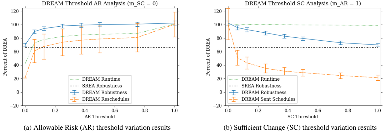
Figure 2: Simulated results for Allowable Risk (AR) and Sufficient Change (SC) on instances from (Lund et al. 2017). We plot the success rate, the mean runtimes, reschedules (a proxy for both computation and communication for AR) and communications (for SC) relative to DREA. We also plot SREA’s robustness to show improvement over the baseline.
