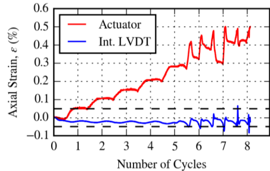
Figure 7. Comparison of axial strain at two locations in the testing apparatus during the cyclic phase of an AC CV-CDSS test ( D_r = 67\% , \sigma'_{v0} = 250 kPa).
