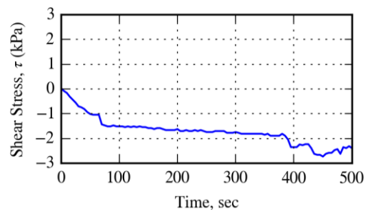
Figure 2. Shear stress during the ramp-up and consolidation phases of a PC CV-CDSS test ( D_r = 23\% , \sigma'_{v0} = 100 kPa).
