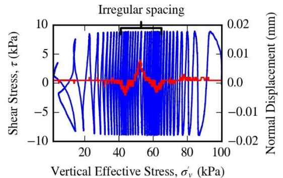
Figure 6. Stress path (in blue) with irregular spacing and normal displacement of the vertical actuator (in red) during a PC CV-CDSS test ( D_r = 20\% ).
