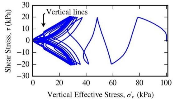
Figure 5. Stress path with vertical lines at low vertical effective stress (PC CV-CDSS test, D_r = 85\% ).
