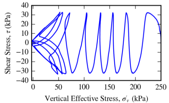
Figure 8. Biased stress path (PC CV-CDSS test, D_r = 67\% ).
