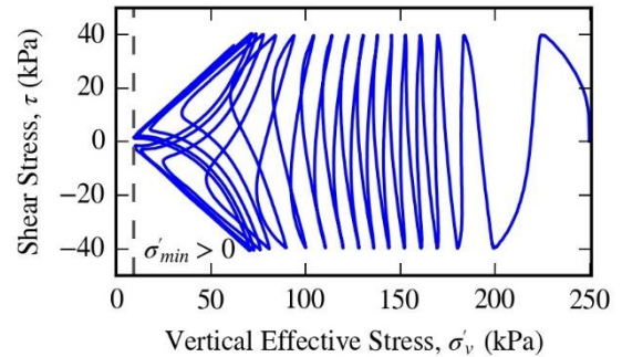
Figure 4. Stress path converging at a non-zero value of vertical effective stress (PC CV-CDSS test, D_r = 70\% ).
