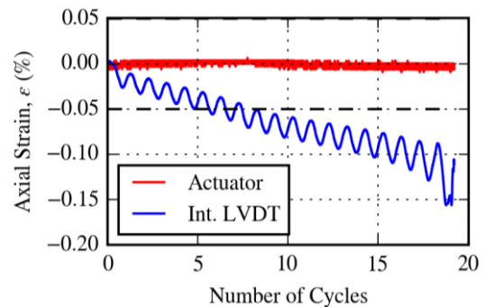
Figure 3. Comparison of axial strain at two locations in the testing apparatus during the cyclic phase of a PC CV-CDSS ( D_r = 19\% , \sigma'_{v0} = 250 kPa).
