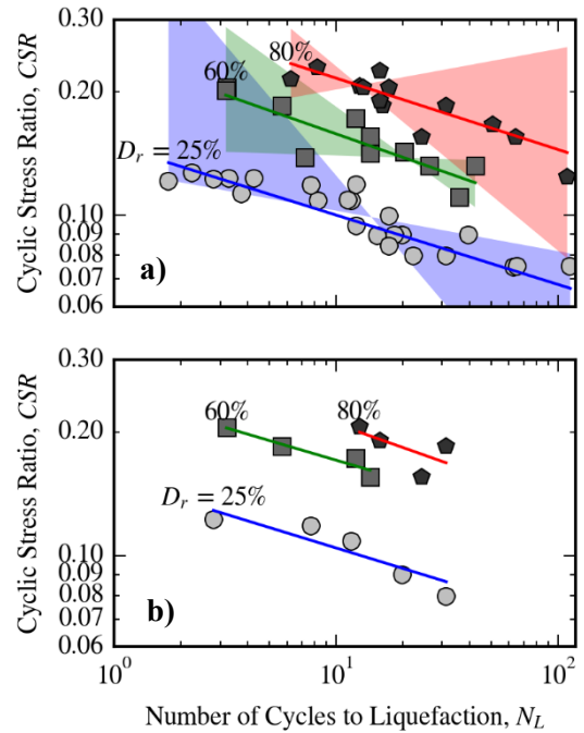
Figure 9. Liquefaction resistance curves (liquefaction defined as single-amplitude \gamma = 3.5\% , \sigma'_{v0} = 100 kPa) for a) all PC CV-CDSS tests, and b) PC CV-CDSS tests that passed the acceptance criteria.
