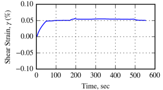
Figure 1. Shear strain during the ramp-up and consolidation phases of a PC CV-CDSS test ( D_r = 58\% , \sigma'_{v0} = 100 kPa).
