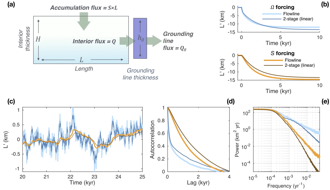
Figure 2. Comparing transient behavior of the flowline and two-stage models. (a) Schematic of the two-stage model. (b) Comparisons of flowline and linearized two-stage model length responses to step changes in \Omega and S . The thinner lines show the two-stage output. (c) Length anomalies in response to white-noise forcing of both types. As in Fig. 1, anomalies have standard deviation of 20% of the mean value and have opposite signs. 5 kyr of the 100 kyr model runs are shown. (d) Autocorrelation function for stochastic length fluctuations. (e) Power spectral density for length fluctuations, which is estimated throughout this study via Welch’s method with windows of 1/16 the timeseries length, and 50% overlap. Note the clear split between fluctuations driven by \Omega' and S' at millennial and shorter timescales. This split is robust across models. The flowline model has more high-frequency power for both types of forcing, but note that the spectral power is orders-of-magnitude lower at such high frequencies.
