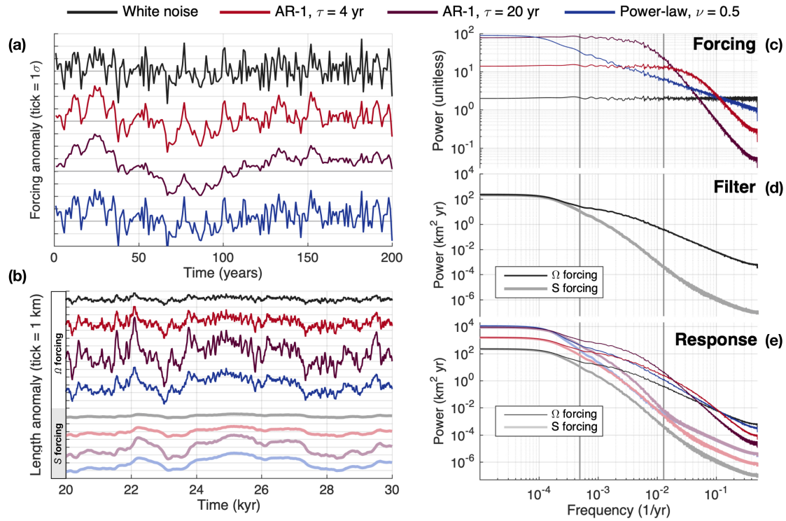
Figure 4. The effect of climatic persistence on glacier fluctuations. (a) Segments of synthetic anomalies with different levels of persistence: white noise (black); 4 yr AR-1 (red); 20 yr AR-1 (maroon); and power-law ( \nu = 0.5 ; blue). Timeseries shown are dimensionless and offset for clarity, with vertical ticks of 1\sigma . (b) The glacier-length variations generated by the two-stage model, when the synthetic anomalies are applied as \Omega' (dark lines) and S' (pastel lines). Timeseries are again offset, with vertical ticks of 1 km. (c) Power spectra of the synthetic climate forcings. For reference, vertical lines correspond to 1/\tau_F and 1/\tau_S . (d) Spectra of the glacier's response to white noise, which illustrates the glacier's sensitivity as a function of frequency, and thus its temporal filtering properties. This depends on whether forcing is applied at the terminus (black) or interior (gray). (e) Spectra of glacier response to each type of synthetic variability, which depend on the spectra of the forcing and glacier's filtering properties. Forcing with persistence has more power at low frequencies where glacier sensitivity is highest, increasing the overall glacier variance.
