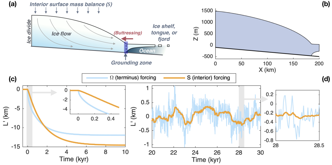
Figure 1. Model schematic and response to forcing. (a) An idealized marine-terminating glacier system. (b) Initial steady-state profile as simulated by the flowline model. (c) Length response to 20% step increase in \Omega (blue) and 20% step decrease in S (orange) at t = 0 . Inset panel zooms into the first 0.5 kyr of response. Note the difference in initial retreat rates depending on the type of forcing. (d) Length response to random, normally-distributed interannual variability in \Omega and S . Anomalies have a standard deviation of 20% of the mean value, and have opposite signs for \Omega and S so that length anomalies will be correlated for comparison. The response to forcing at the grounding line ( \Omega ) contains much more high-frequency content.
