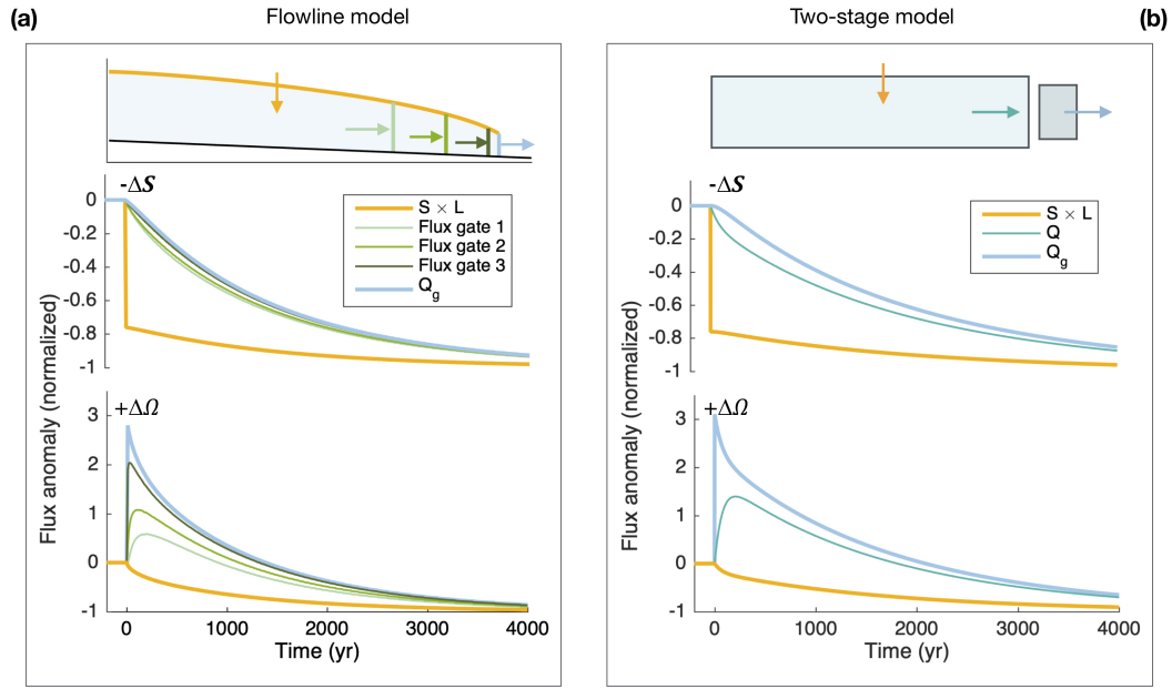
Figure 3. Flux changes following interior vs. grounding-zone forcings. (a) Flowline model flux anomalies to perturbations in S and \Omega . The schematic (top) shows the flux gates considered. Below, normalized flux responses to the perturbations are shown for each flux gate. (b) as for (a), but for the two-stage model, which has three flux variables. The two-stage model's interior flux variable ( Q ) captures the basic tendencies of interior fluxes in the flowline model. In both cases, the response to a perturbation in \Omega clearly shows the two-timescale nature of outlet glacier dynamics.
