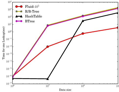
Figure 9. Point lookup latency relative to data size.
