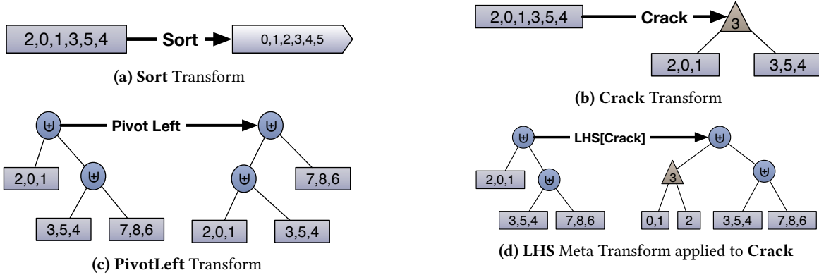
Figure 5. Example of transformations over COG
