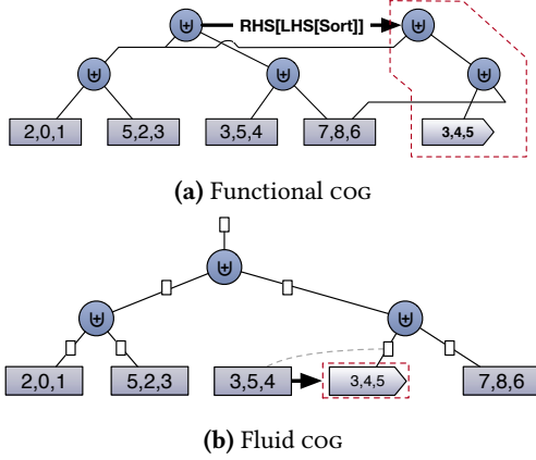
Figure 6. Applying the transform \text{RHS}[\text{LHS}[\text{Sort}]] to instances of both Functional cog and Fluid cog.
