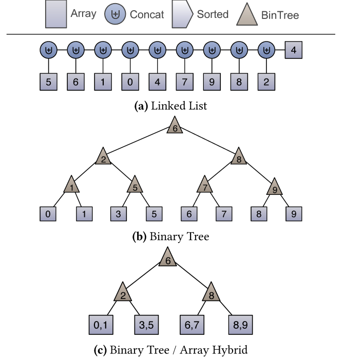
Figure 3. Example abstract syntax trees for three logically equivalent, correct sentences in cog.
