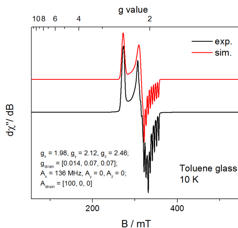
Figure 2. X-band EPR Spectrum of ( R,R )-(BenzP*)Co(COD) Recorded in Toluene Glass at 10 K. Microwave frequency = 9.38 GHz, power = 0.02 mW and modulation amplitude = 0.4 mT/100 kHz. Simulation of EPR signal supports an S = ½ ground state. Simulation parameters: g x = 1.98, g y = 2.12, g z = 2.46, g strain = [0.014, 0.07, 0.07], A x = 136 MHz, A y = 0, A z = 0, A strain = [100, 0, 0].
