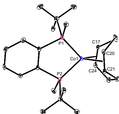
Figure 1. Solid-state structure of ( R,R )-(BenzP*)Co(COD) at 30% probability ellipsoids with hydrogen atoms omitted for clarity. Selected bond distances(angstrom): Co1–C17, 2.062(5), Co1–C20, 2.114(5), Co1–C21, 2.141(5), Co1–C24, 2.048(4), C20–C21, 1.386(6), C17–C24, 1.409(7).
