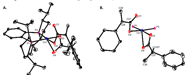
Figure 5. A. Solid State Structure of (Λ)-( R,R )-(iPr 2 DuPhos)Co(κ 1 -O 2 C-C 8 H 7 )(κ 2 -O 2 C-C 8 H 9 ) at 30% Probability Ellipsoids with H atoms Omitted for Clarity. B. Truncated View at 30% Probability Ellipsoids with H atoms (except H37) Omitted for Clarity. Bond lengths: C28–C29 = 1.336(9) Å, C37–C38 = 1.47(2) Å, Bond angles (avg.): center at C28, 120.0(1)°, center at C37, 111.5(1)°.
