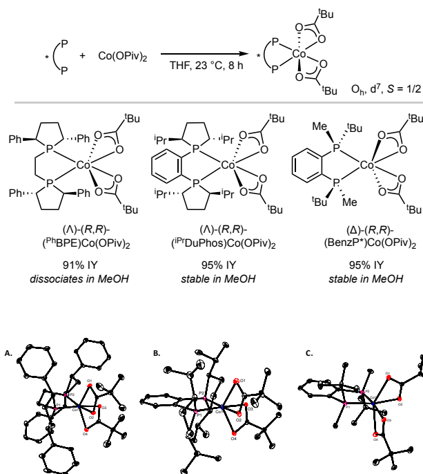
Figure 3. Solid State Structure of A. (Λ)-(R,R)- Ph BPE)Co(OPiv) 2 B. (Λ)-(R,R)-( iPr DuPhos)Co(OPiv) 2 C. (Δ)-(R,R)-(BenzP*)Co(OPiv) 2 at 30% Probability Ellipsoids with H Atoms Omitted for Clarity.
