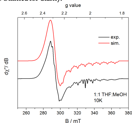
Figure 4. X-band EPR Spectrum of (R,R)-(BenzP*)Co(OPiv) 2 Recorded in 1:1 THF:MeOH Glass at 10 K. Microwave frequency = 9.38 GHz, power = 0.02 mW and modulation amplitude = 0.4 mT/100 kHz. Simulation of EPR signal supports an S = 1/2 ground state. Simulation parameters: g x = 2.01, g y = 2.27, g z = 2.32, g strain = [0.0126, 0.0510, 0.120]. A Co x = 246 MHz, A Co y = 0, A Co z = 0, A P1 x = A P2 x = 80 MHz, A P y = 0, A P z = 0.
