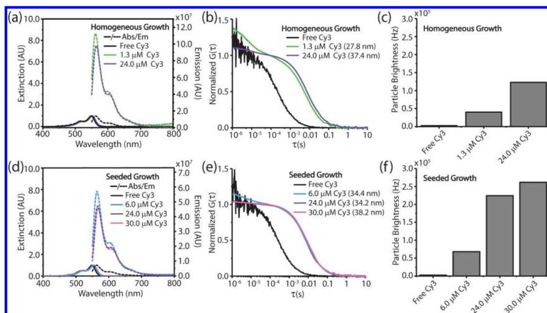
Figure 3. Characterization of fluorescent SNPs synthesized by (a–c) homogeneous and (d–f) seeded growth. (a,d) Absorbance (solid lines) and emission spectra (dashed lines), (b,e) FCS curves, and (c,f) FCS-derived per particle brightness values for SNPs synthesized using homogeneous or seeded growth and varying Cy3/APTES or Cy3/AEAPTMS concentrations, respectively. The emission spectra in (a) and (d) are truncated on the left side because of overlap with the 543 nm excitation source prevents direct quantification of the sample emission at these wavelengths. Noise levels of FCS curves for free dye in (b) and (e) are higher than for particles due to substantially increased particle brightness, see (a) and (d).
