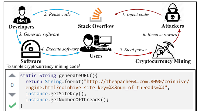
Figure 1: Example of code security attacks in Stack Overflow.
