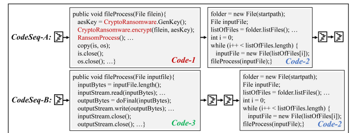
Figure 4: Different contexts among code snippets.
