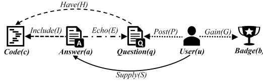
Figure 3: Network schema for HIN in our application.
