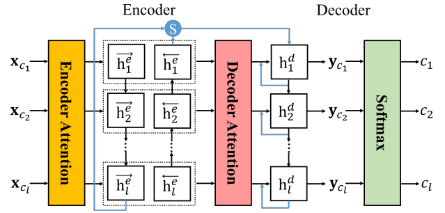
Figure 5: Architecture of LSTM using hierarchical attention.
