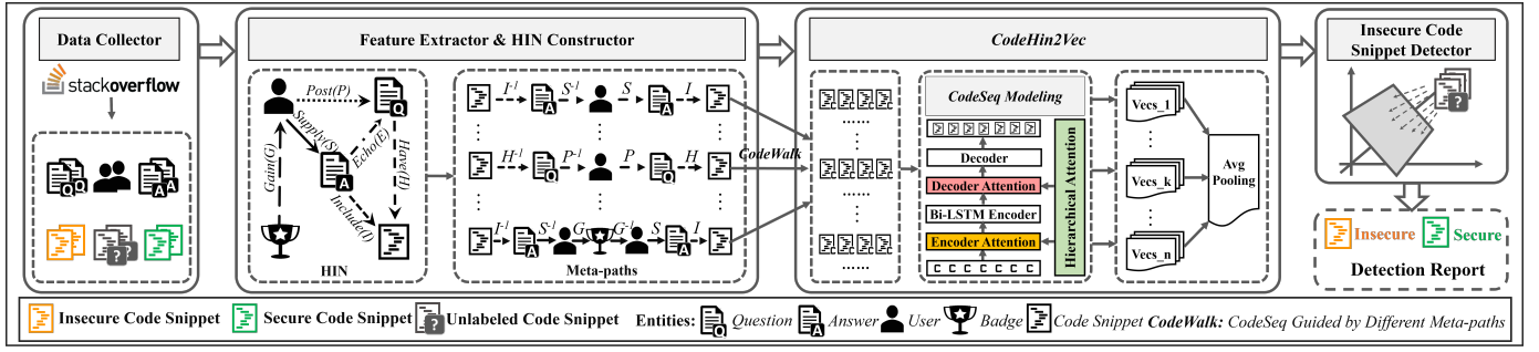
Figure 2: System architecture of iTrustSO .
