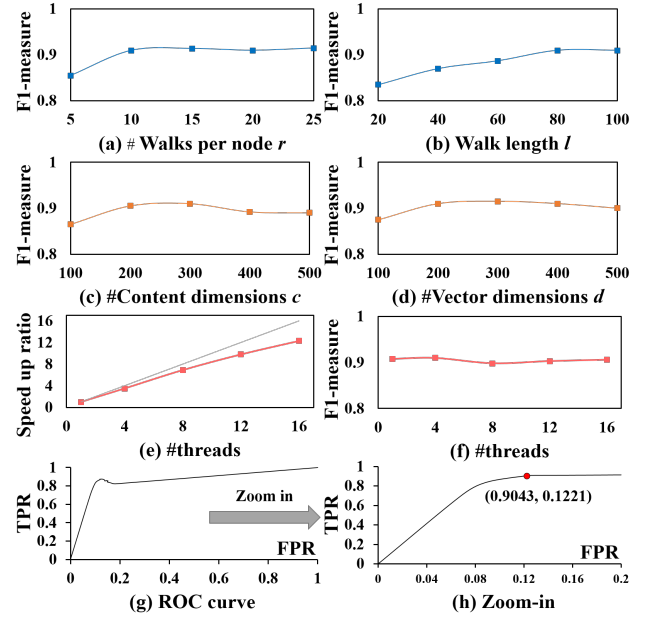
Figure 7: Parameter sensitivity evaluation.
