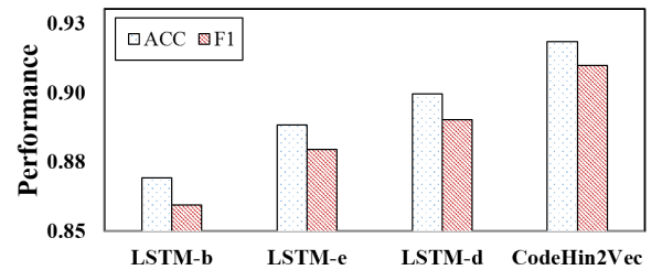
Figure 6: Attention evaluation.
