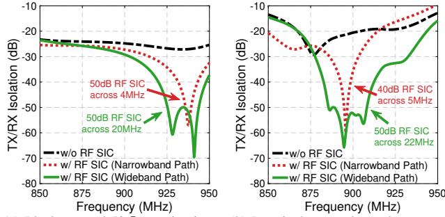
(a) Ideal case w/ 50\ \Omega termination. (b) Practical case w/ a real antenna. Fig. 3: Measured TX/RX isolation of the Gen-2 RF canceller without turning on the canceller, and with the narrowband (Gen-1)/wideband (FDE) path on, when the circulator antenna port is: (a) terminated by 50\ \Omega , and (b) connected to an antenna.
