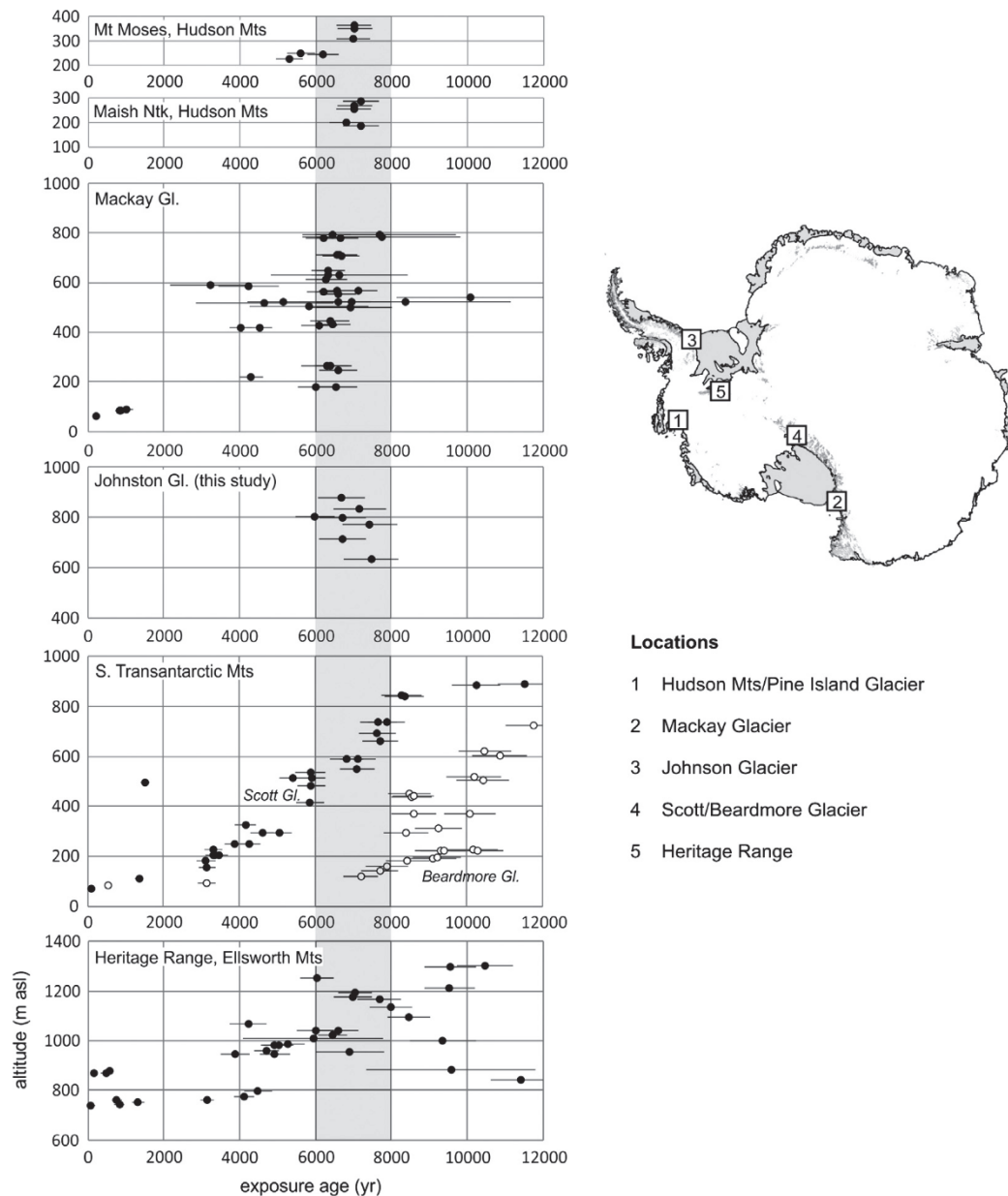
Fig. 6. Holocene thinning histories derived from exposure age dating from selected sites in Antarctica (Hudson Mountains/Pine Island Glacier, Johnson et al., 2014; Mackay Glacier, Jones et al., 2015; Johnston Glacier, this study; Scott and Beardmore Glaciers, southern Transantarctic Mountains, Spector et al., 2017; Heritage Range, Ellsworth Mountains; Hein et al., 2016). Exposure ages shown are all ^{10}\text{Be} , with the exception of Johnston Glacier where deglaciation ages were determined using in situ ^{14}\text{C} . Vertical axes are altitude (m asl) and horizontal axes are exposure age (yr). All data shown are publicly accessible on the ICE-D:Antarctica database ( http://antarctica.ice-d.org ). The upper five panels show locations where episodes of rapid thinning occurred at 6–8 ka (time period indicated by grey shading).
