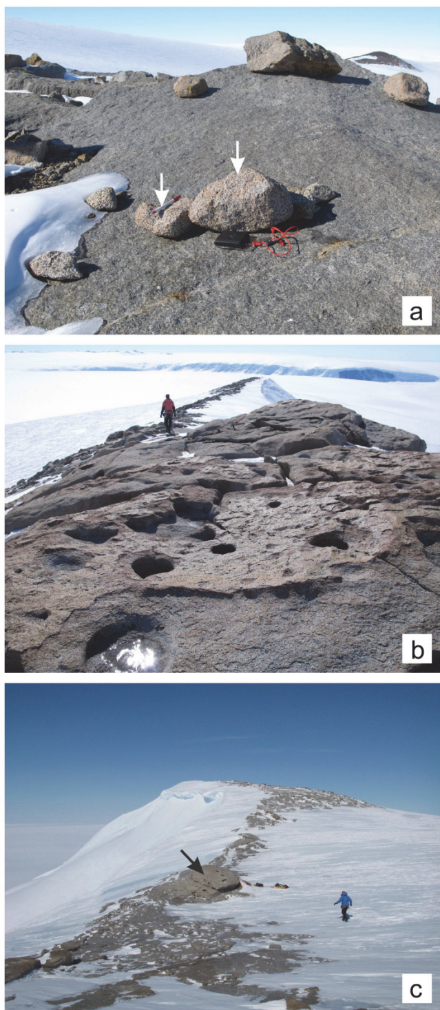
Fig. 2. Surface features on nunataks of the Bowman Peninsula, Lassiter Coast. (a) Sub-angular granodiorite erratic cobbles – indicated by arrows – perched on smooth bedrock surfaces of the same lithology. Compass and pen for scale. Photograph location: -74.5027^{\circ}\text{S}/-62.5664^{\circ}\text{W} (b) Bedrock surface with abundant weathering pits. Smith Peninsula (situated NE of Bowman Peninsula; Fig. 1b) is visible in the background. Person for scale. Location: -74.5434^{\circ}\text{S}/-62.4229^{\circ}\text{W} (c) Small tor-like feature – marked with an arrow – with weathering pits on its uppermost surface, formed in granodiorite bedrock. Person for scale. Location: -74.5535^{\circ}\text{S}/-62.4703^{\circ}\text{W} .
