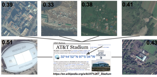
Figure 6: The cosine similarities between the CNN embeddings and the Doc2Vec embedding are computed and overlaid on the images. The CNN learns to embed AT&T Stadium’s image closer to the its corresponding article.
