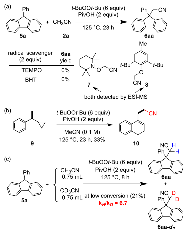
Scheme 6. Control Experiments
